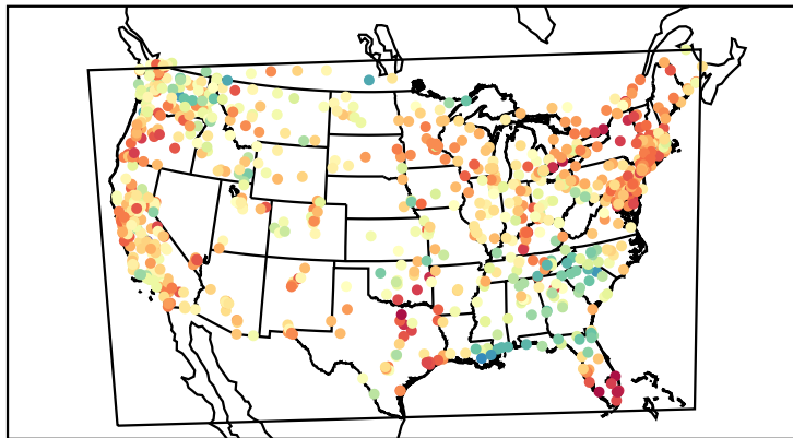
Correlation Coefficient (20190715)
