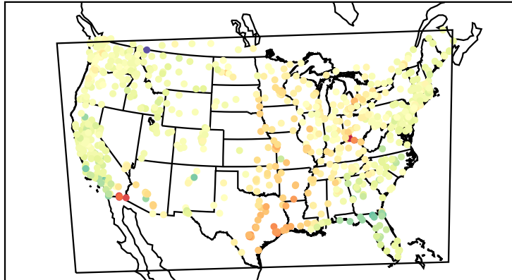
Mean Bias (20190715)
