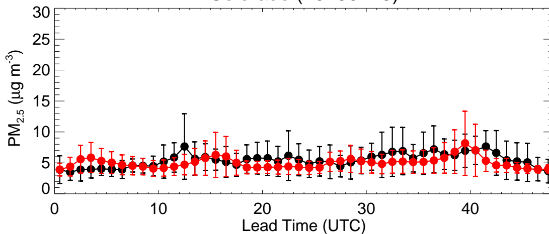
Colorado (20190715)
