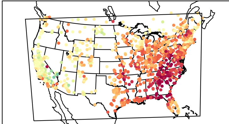
Mean Bias (20190716)
