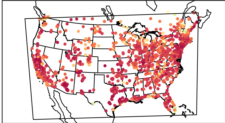
Correlation Coefficient (20190716)
