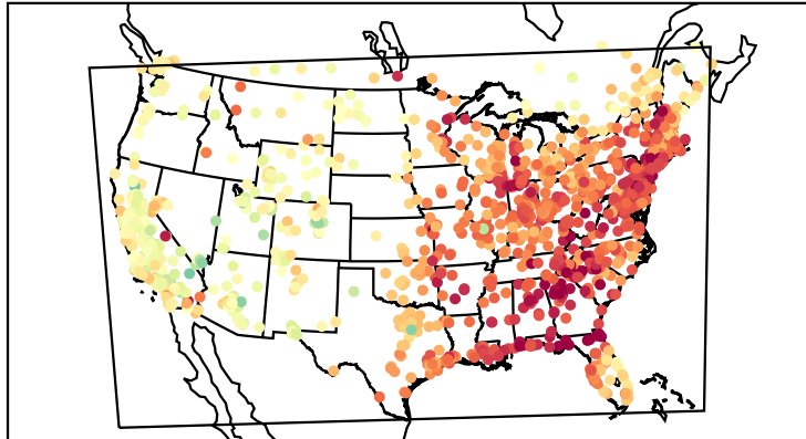
Mean Bias (20190717)
