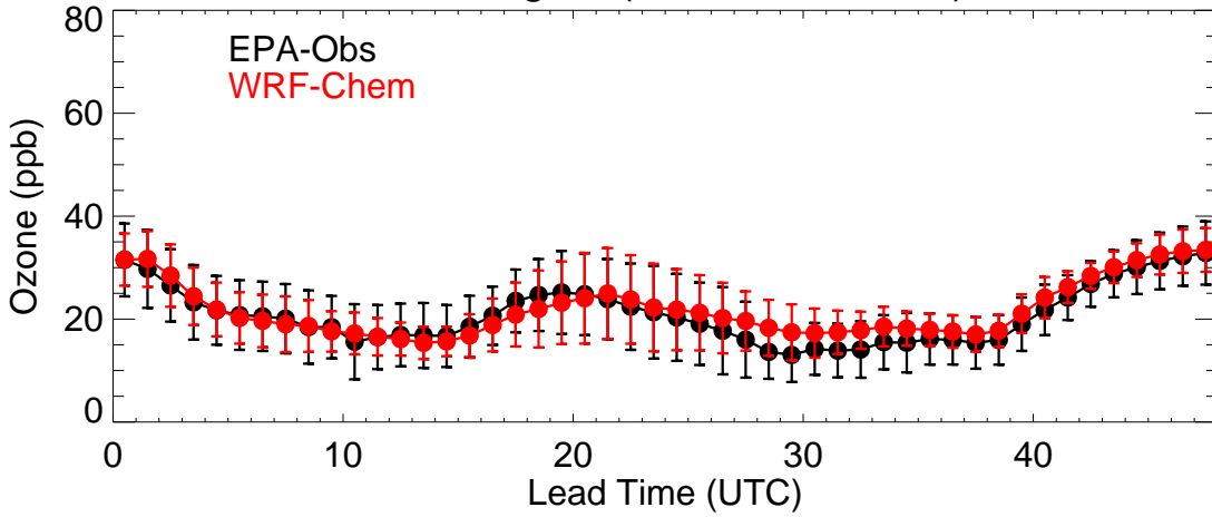
Colorado (20190717)
