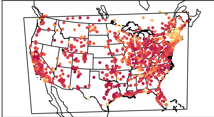
Correlation Coefficient (20190717)
