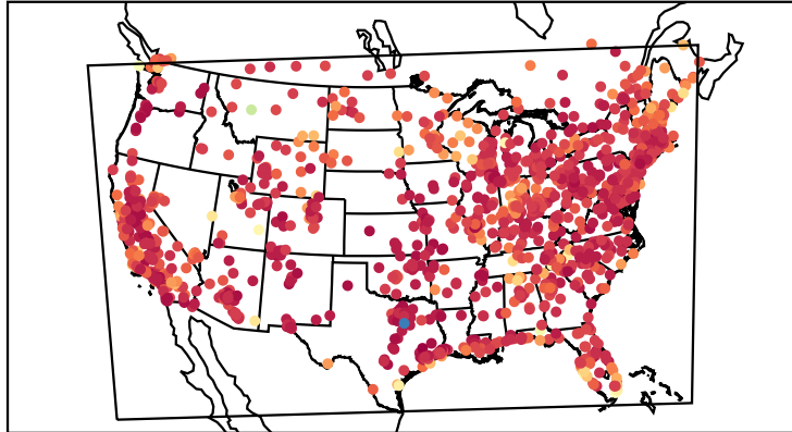
Correlation Coefficient (20190718)
