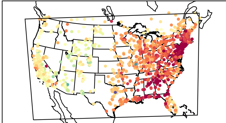
Mean Bias (20190718)
