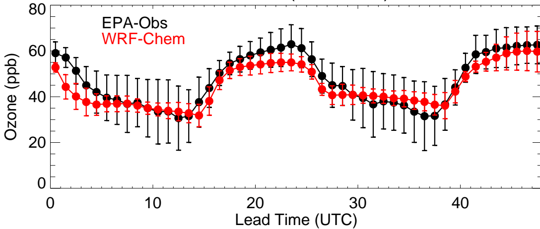
Colorado (20190718)
