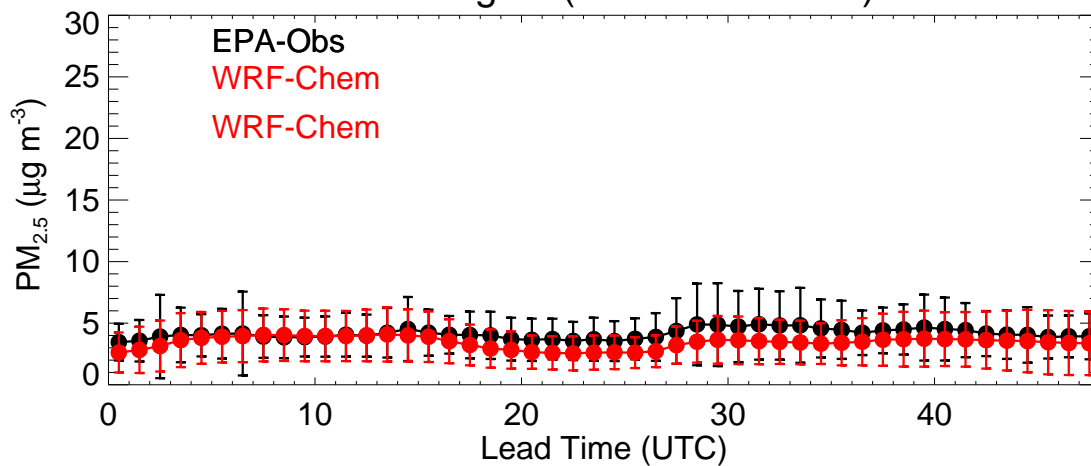
Colorado (20190719)
