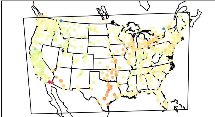
Mean Bias (20190719)
