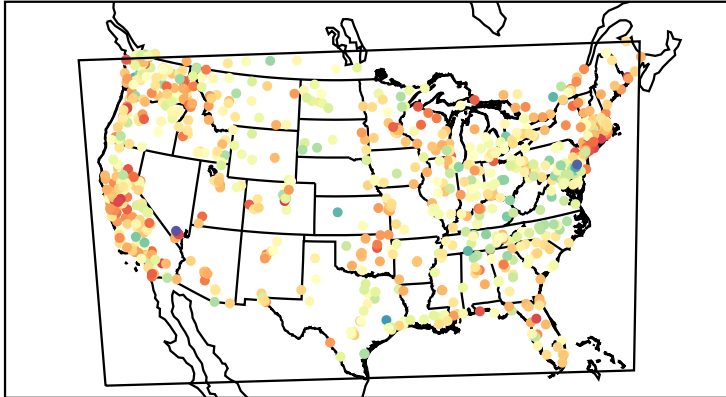
Correlation Coefficient (20190719)
