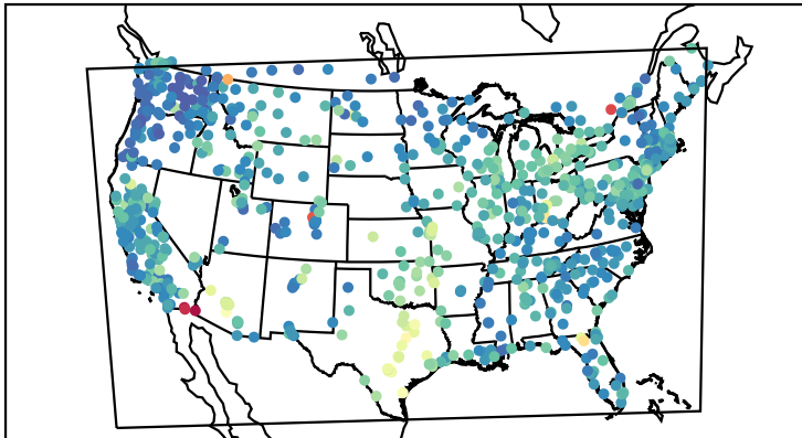
Root Mean Square Error (20190719)
