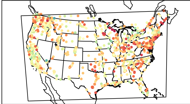
Correlation Coefficient (20190721)
