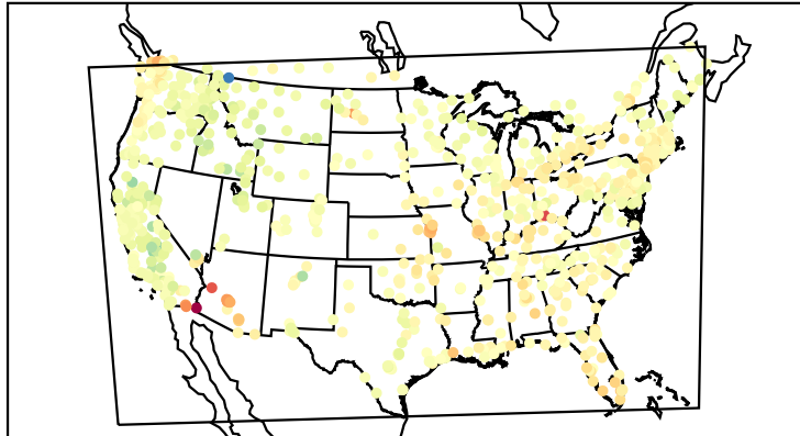
Mean Bias (20190721)
