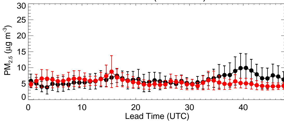
Colorado (20190721)
