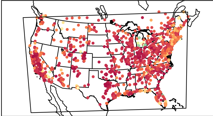
Correlation Coefficient (20190723)
