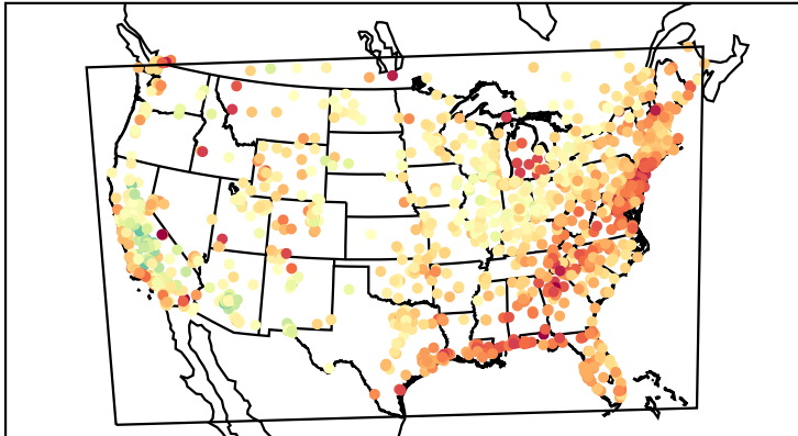
Mean Bias (20190723)
