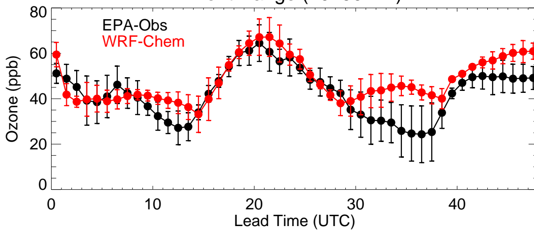
Front Range (20190727)
