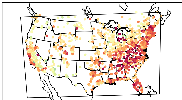
Mean Bias (20190727)
