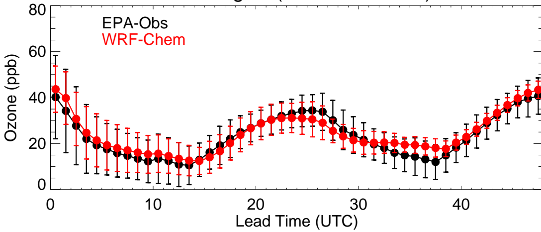
Colorado (20190727)
