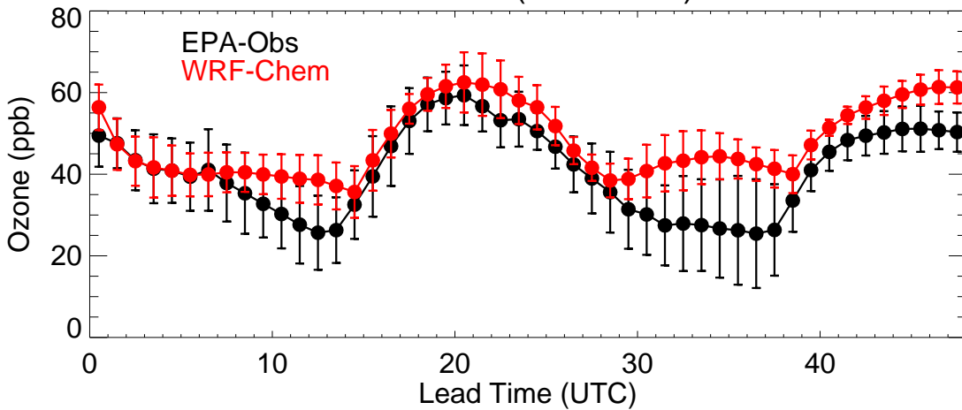
Colorado (20190727)
