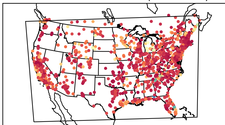
Correlation Coefficient (20190727)
