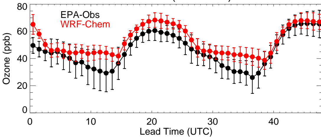
Colorado (20190805)
