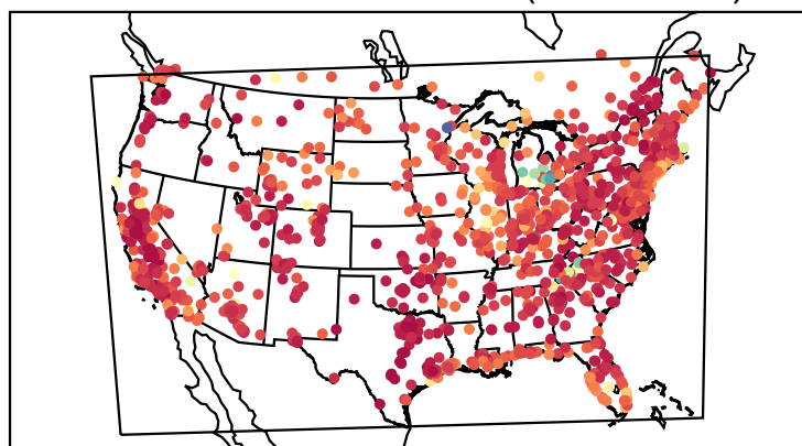
Correlation Coefficient (20190805)
