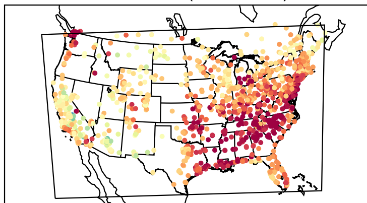
Mean Bias (20190805)
