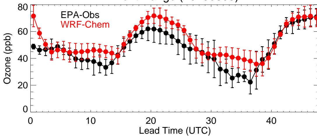
Front Range (20190805)
