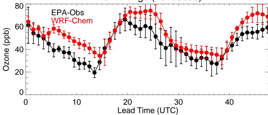
Front Range (20190808)
