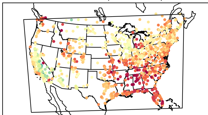
Mean Bias (20190808)
