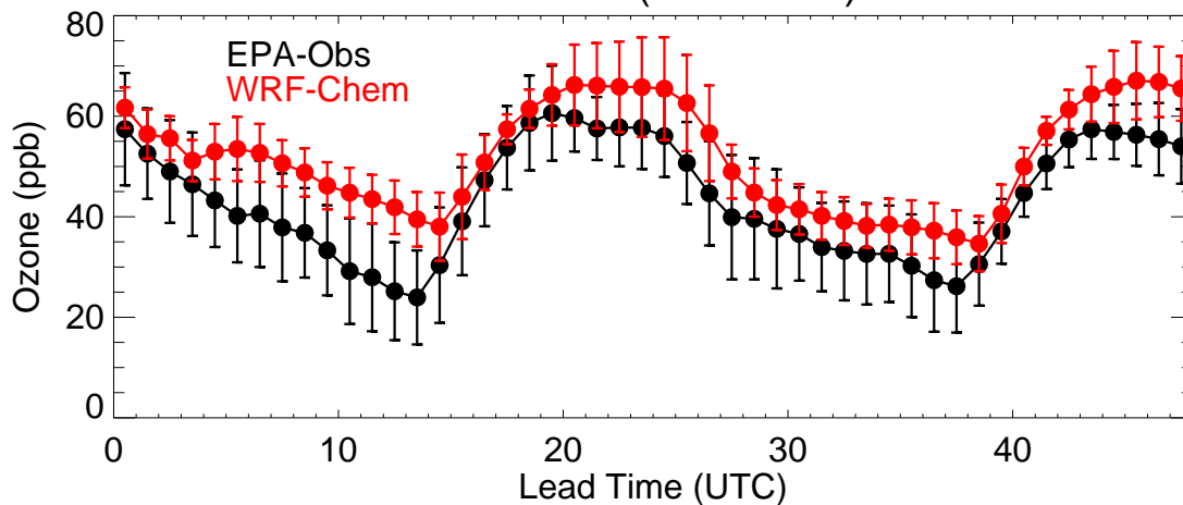
Colorado (20190808)
