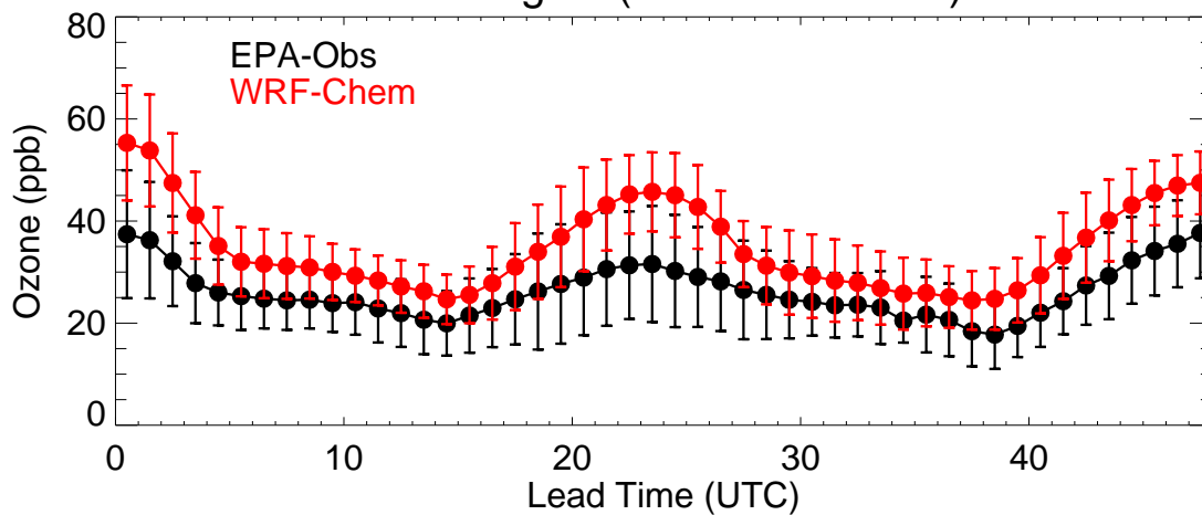
Colorado (20190808)
