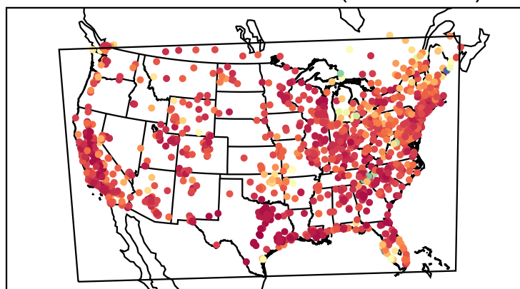
Correlation Coefficient (20190808)
