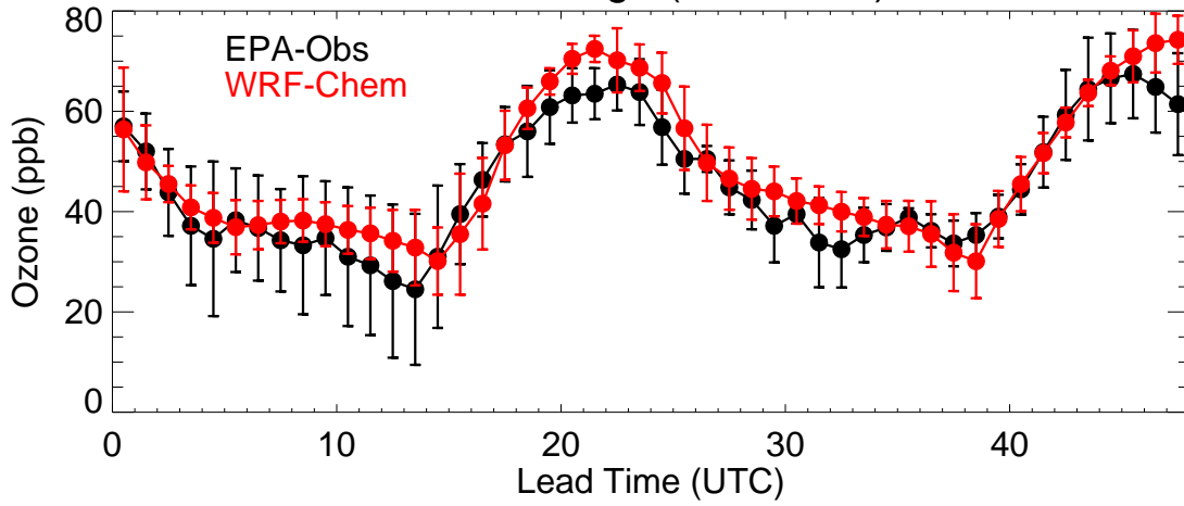
Front Range (20190820)
