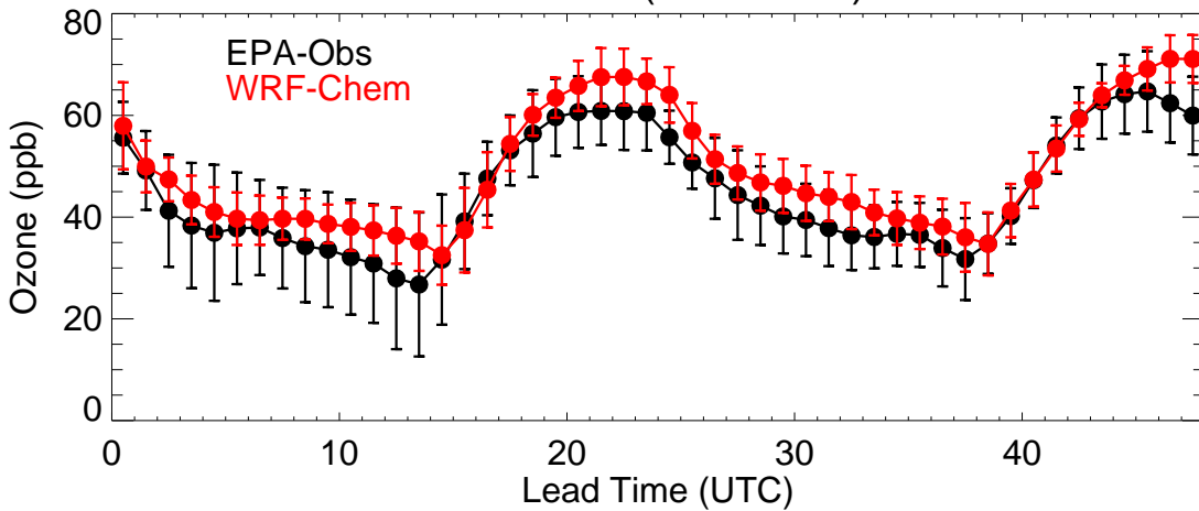
Colorado (20190820)
