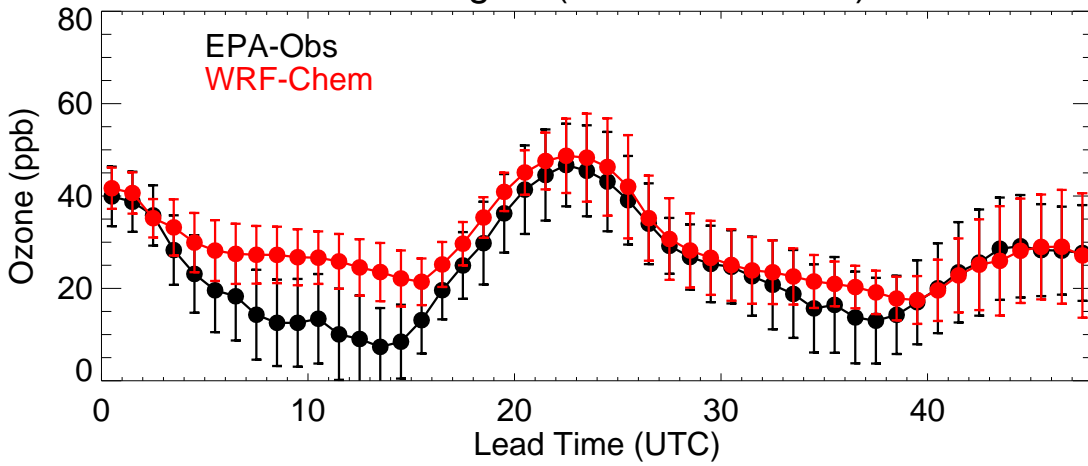
Colorado (20190820)
