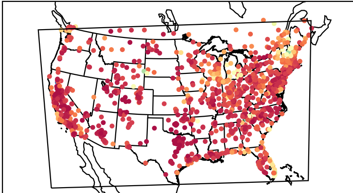
Correlation Coefficient (20190820)
