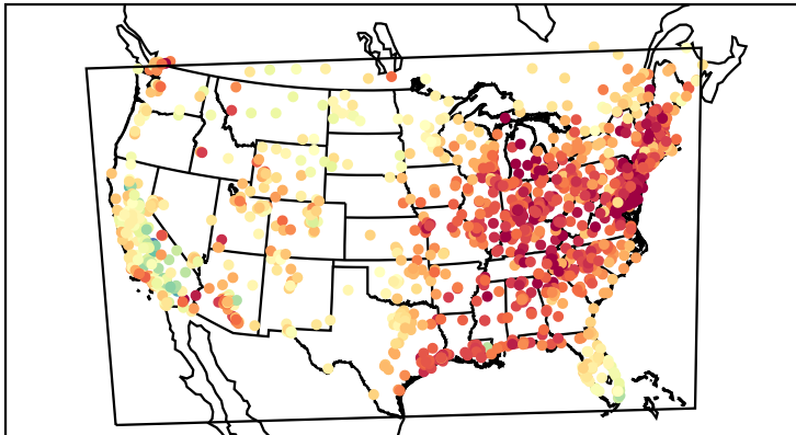
Mean Bias (20190820)
