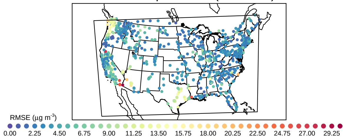
Root Mean Square Error (20190824)
