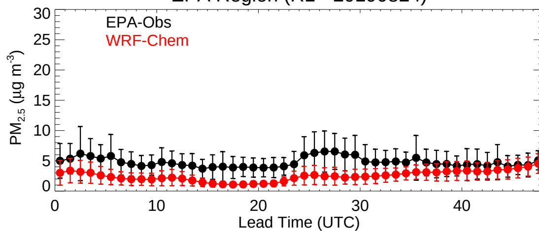
EPA Region (R2 - 20190824)
