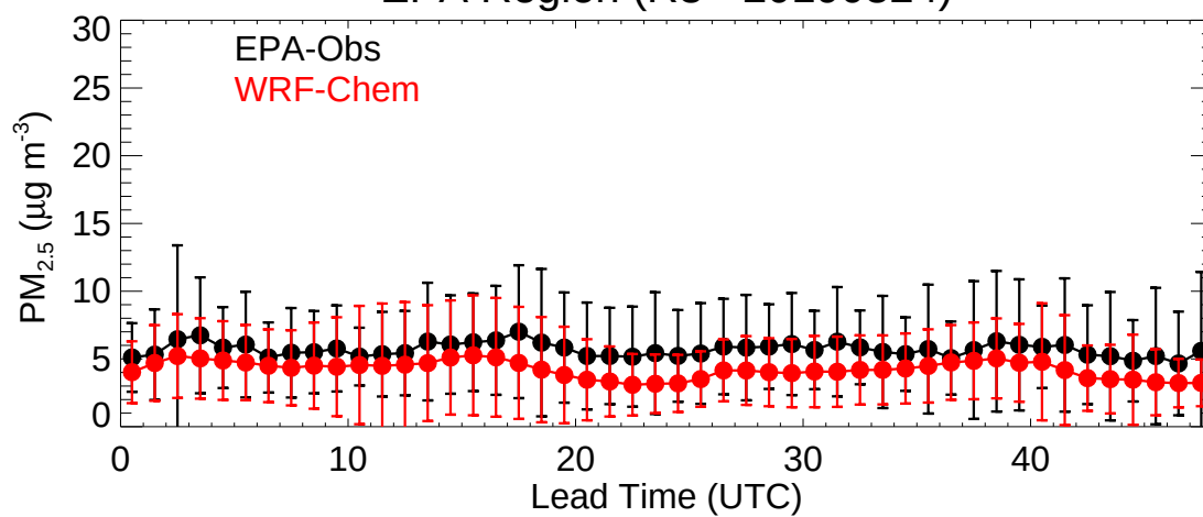
EPA Region (R8 - 20190824)
