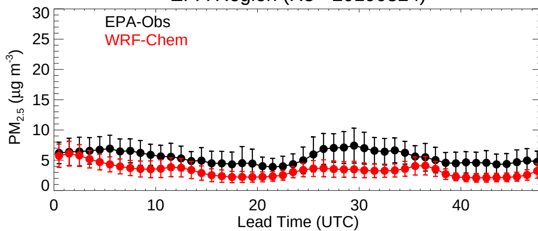
EPA Region (R4 - 20190824)
