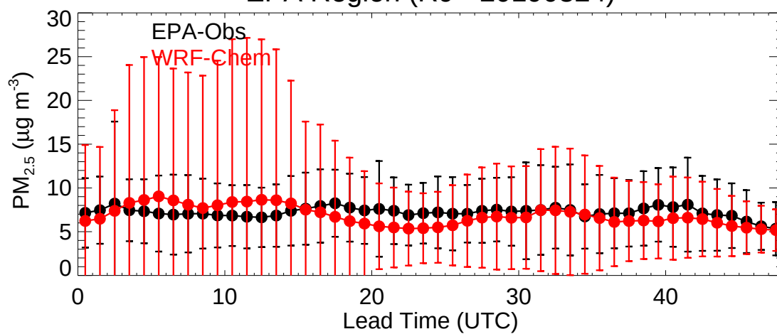
EPA Region (R10 - 20190824)
