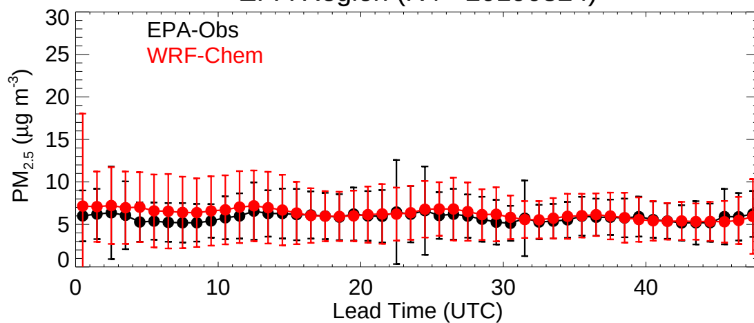
EPA Region (R5 - 20190824)
