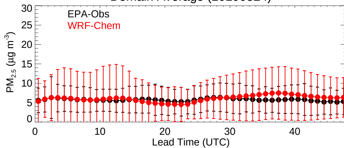
EPA Region (R1 - 20190824)
