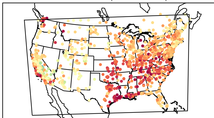
Mean Bias (20190831)
