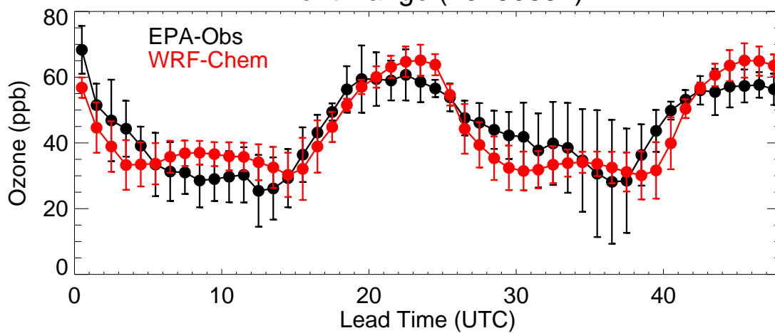
Front Range (20190831)
