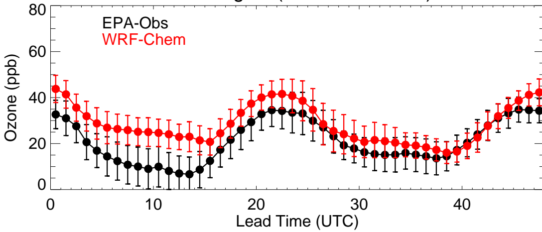
Colorado (20190831)
