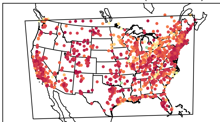
Correlation Coefficient (20190831)
