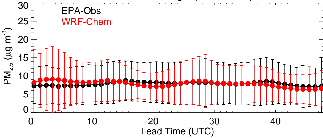
EPA Region (R1 - 20190911)
