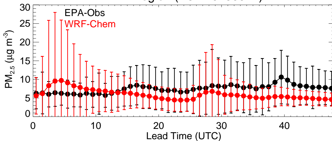
EPA Region (R10 - 20190911)
