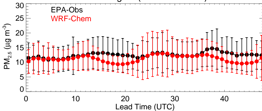
EPA Region (R5 - 20190911)
