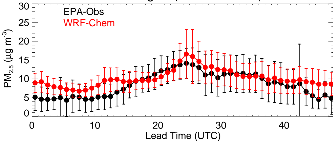
EPA Region (R2 - 20190911)
