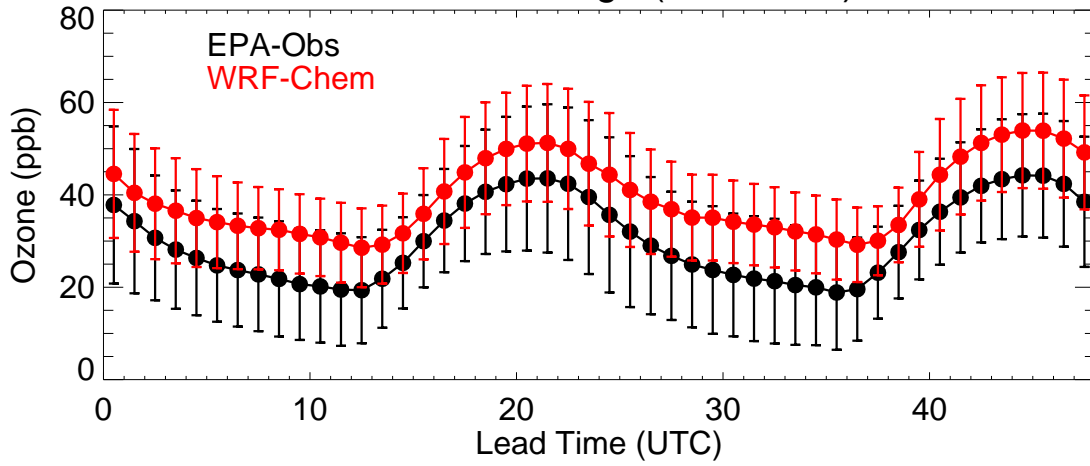
EPA Region (R1 - 20190914)
