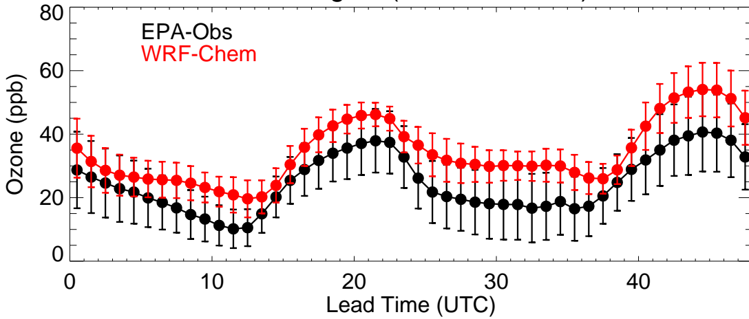
EPA Region (R5 - 20190914)
