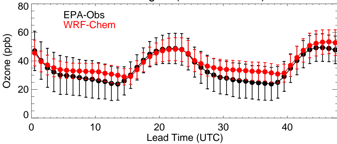
EPA Region (R8 - 20190914)
