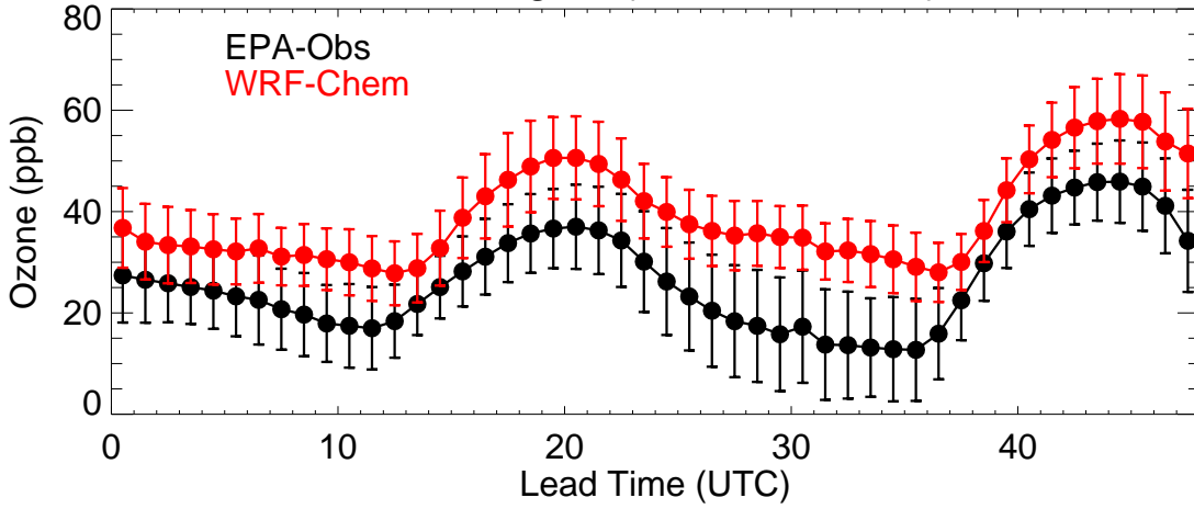
EPA Region (R4 - 20190914)
