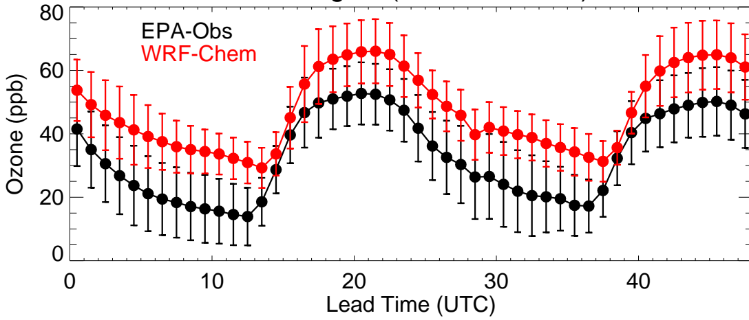
EPA Region (R7 - 20190914)
