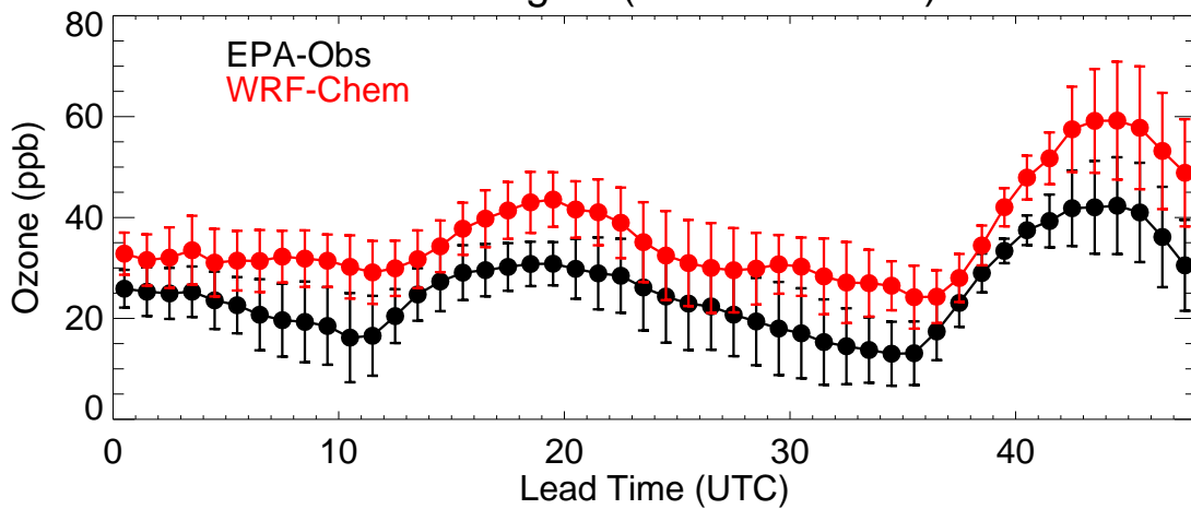
EPA Region (R2 - 20190914)
