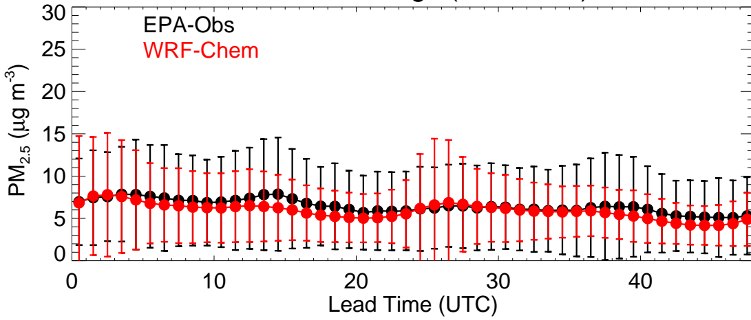
EPA Region (R1 - 20191003)
