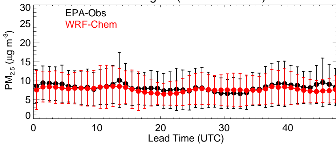
EPA Region (R7 - 20191003)
