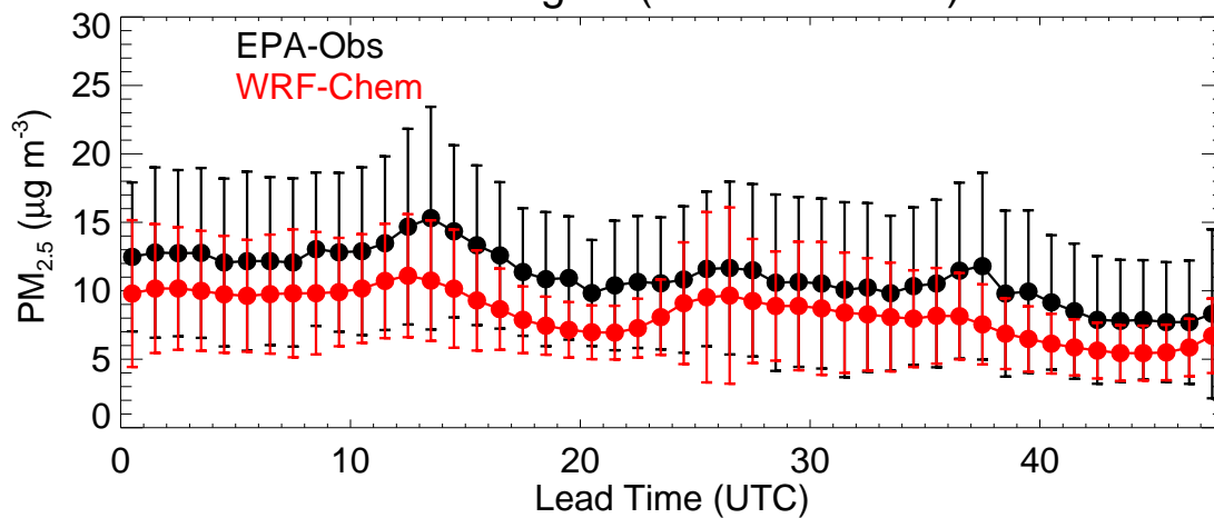
EPA Region (R5 - 20191003)
