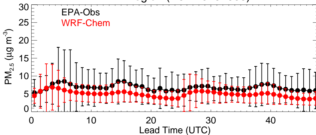
EPA Region (R10 - 20191003)
