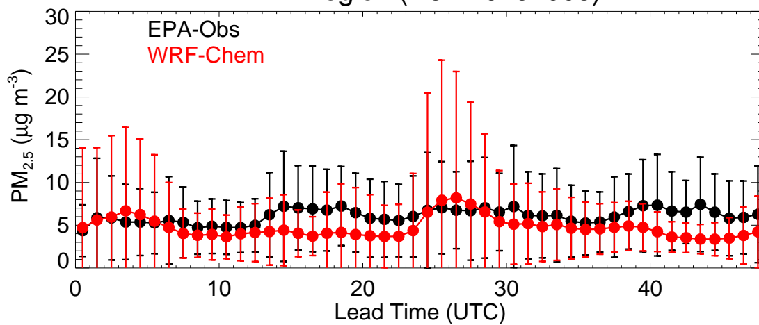
EPA Region (R8 - 20191003)
