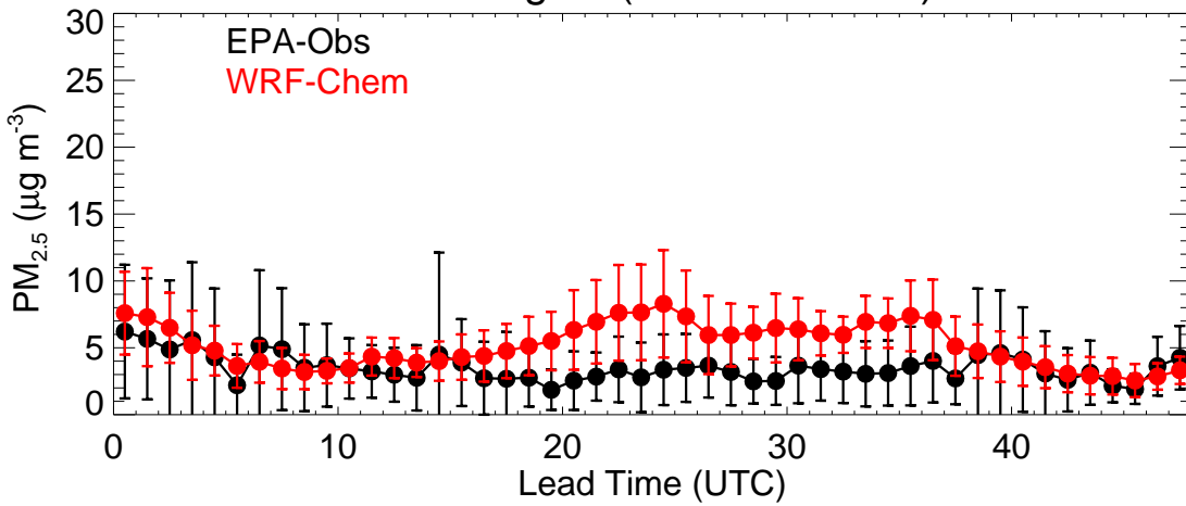
EPA Region (R2 - 20191003)
