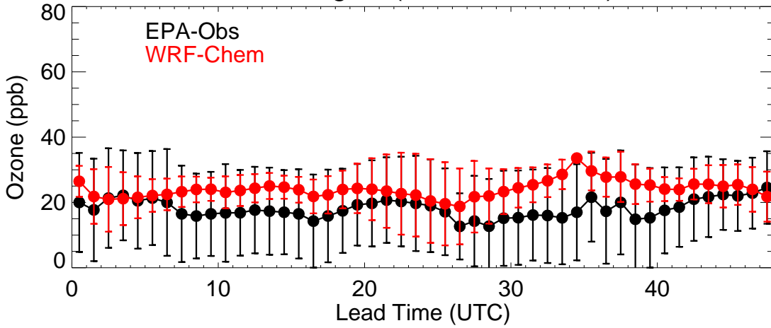
Colorado (20191116)
