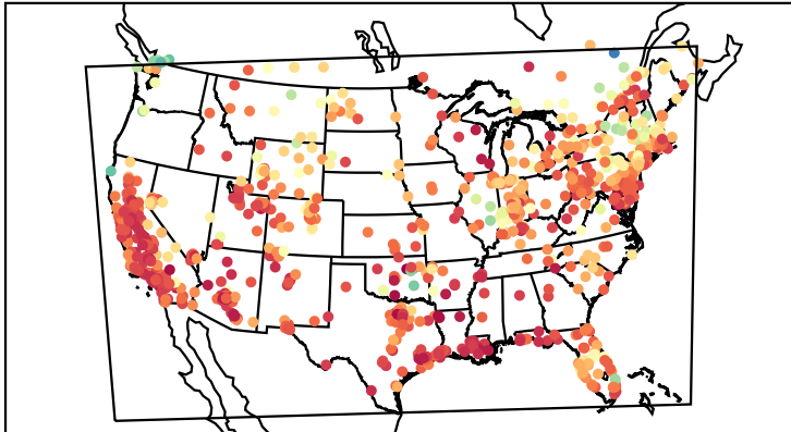
Correlation Coefficient (20191116)
