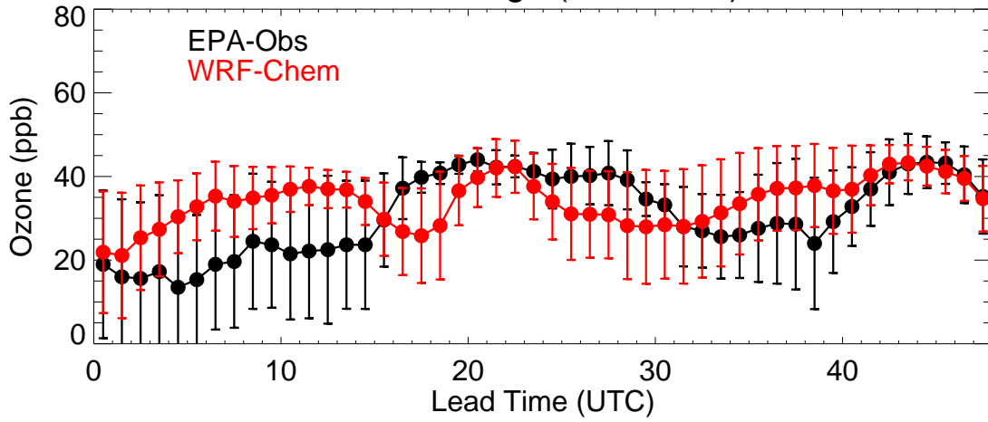
Front Range (20191116)
