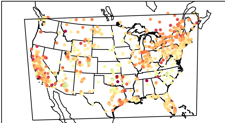
Mean Bias (20191116)
