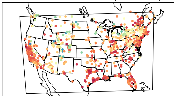
Correlation Coefficient (20191223)
