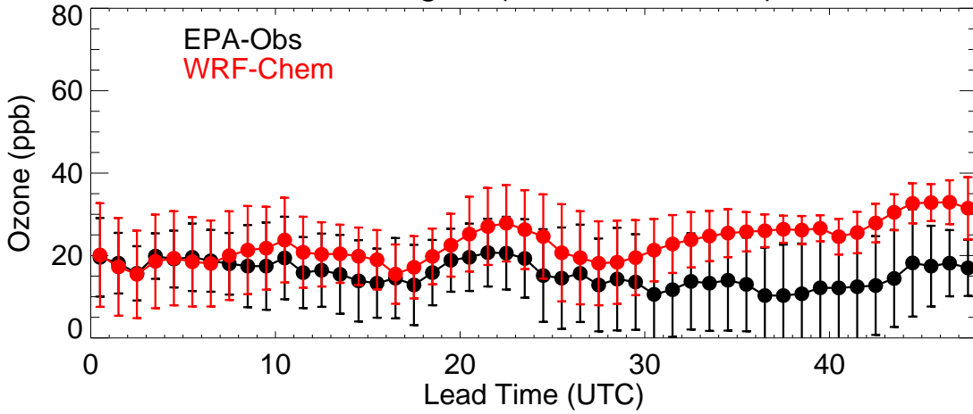
Colorado (20191223)
