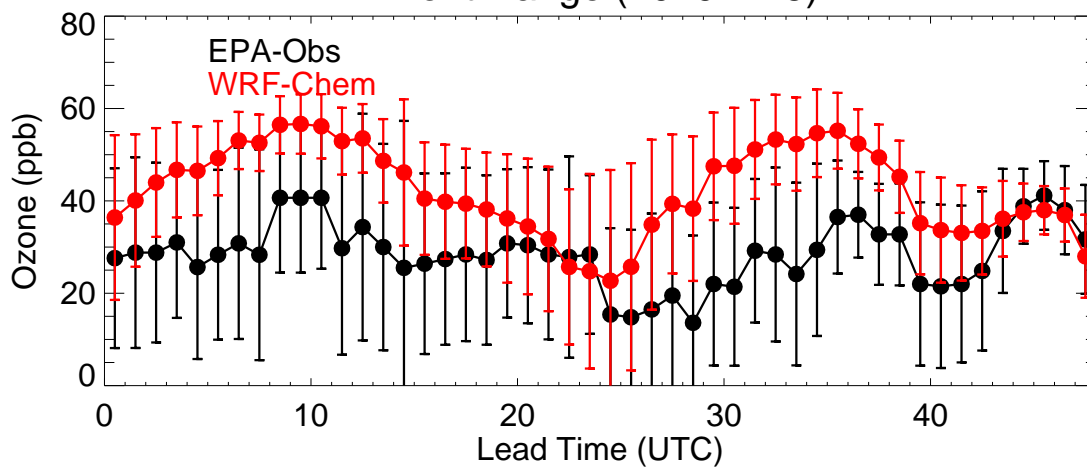
Front Range (20191223)
