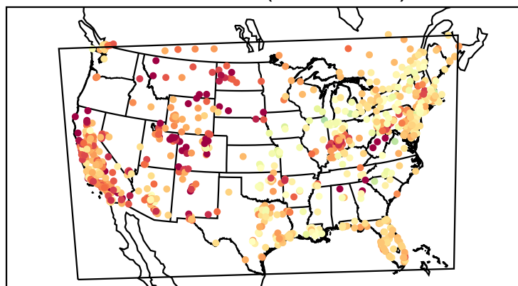
Mean Bias (20191223)
