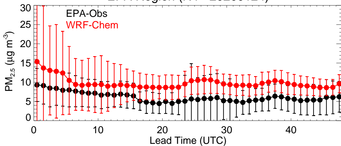
EPA Region (R5 - 20200124)
