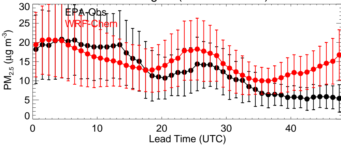
EPA Region (R2 - 20200124)
