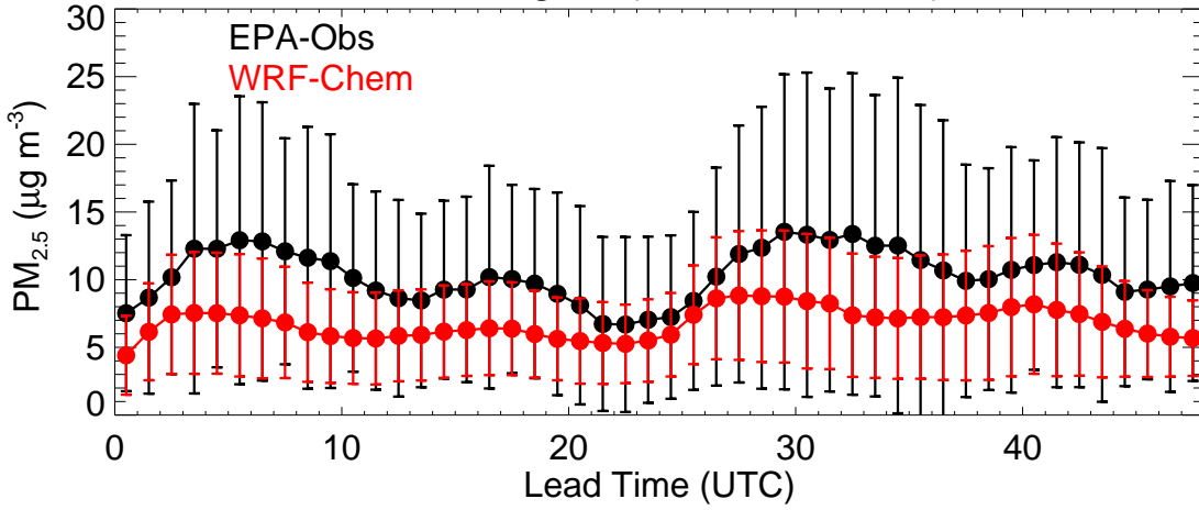
EPA Region (R10 - 20200124)
