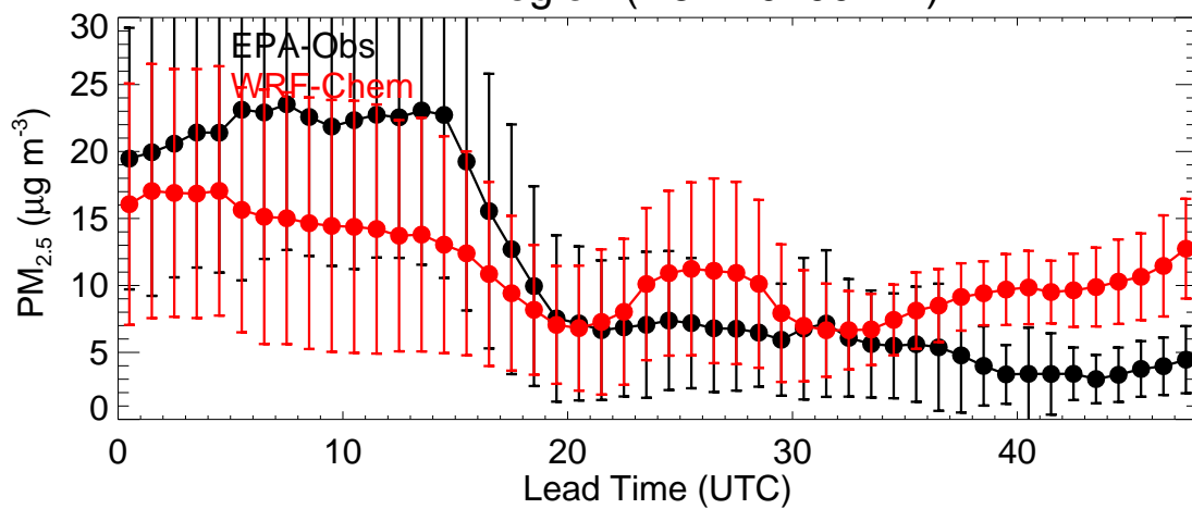
EPA Region (R4 - 20200124)
