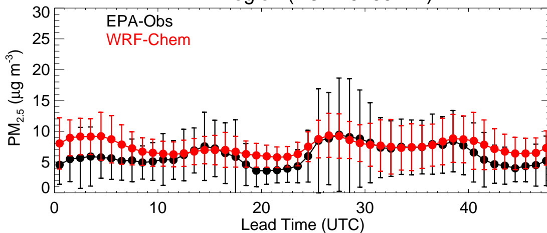
EPA Region (R7 - 20200124)
