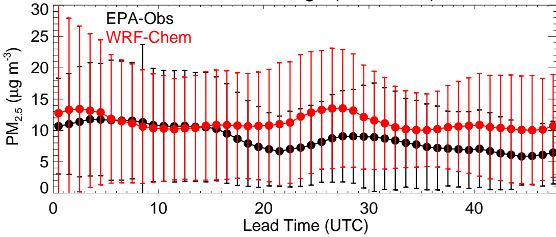
EPA Region (R1 - 20200124)
