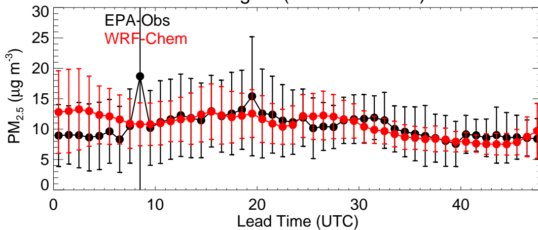
EPA Region (R8 - 20200124)
