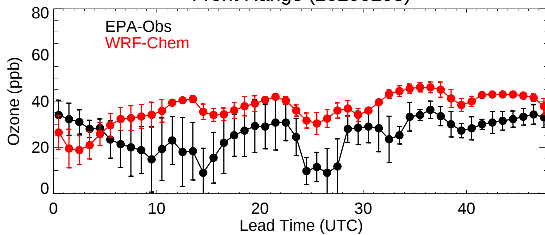
Front Range (20200208)
