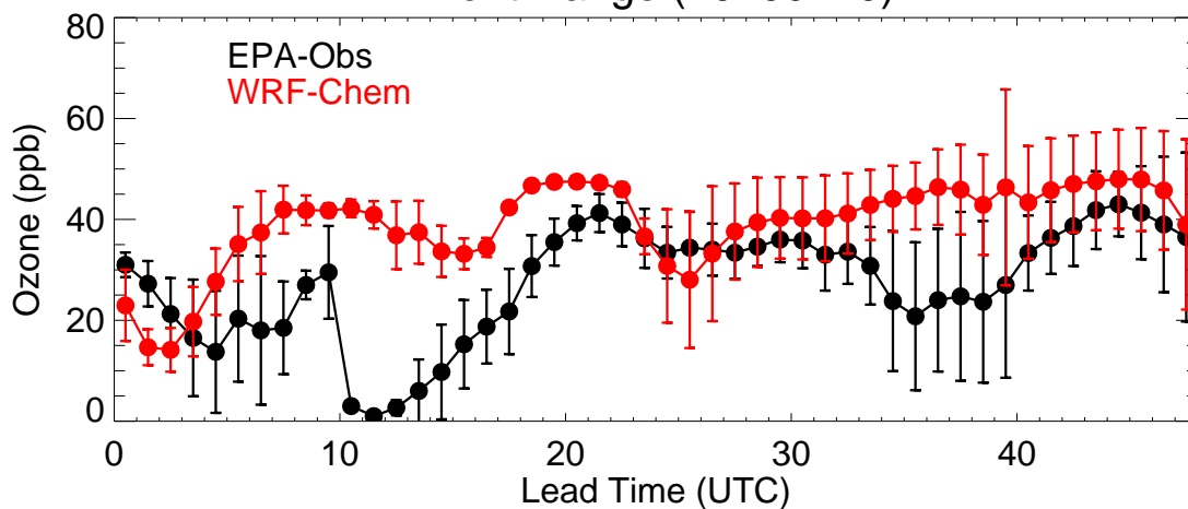
Front Range (20200210)
