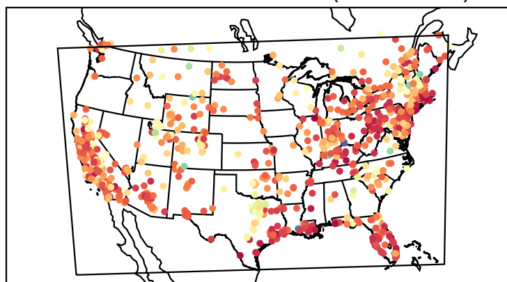
Correlation Coefficient (20200210)
