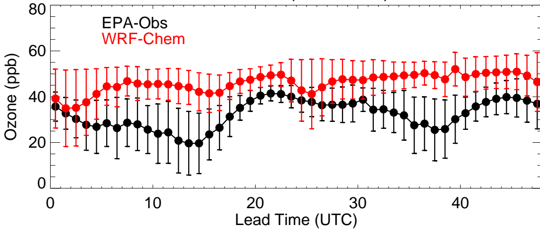
Colorado (20200210)
