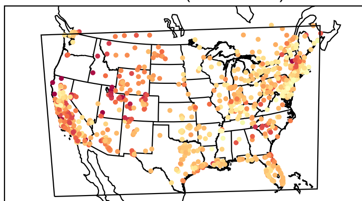
Mean Bias (20200210)
