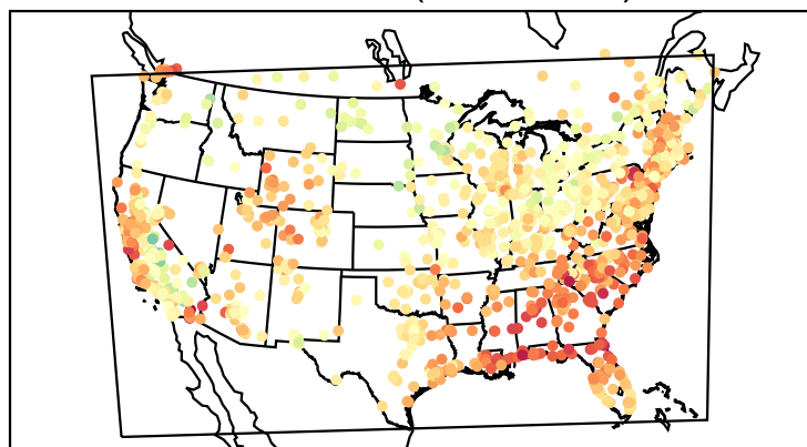
Mean Bias (20200626)
