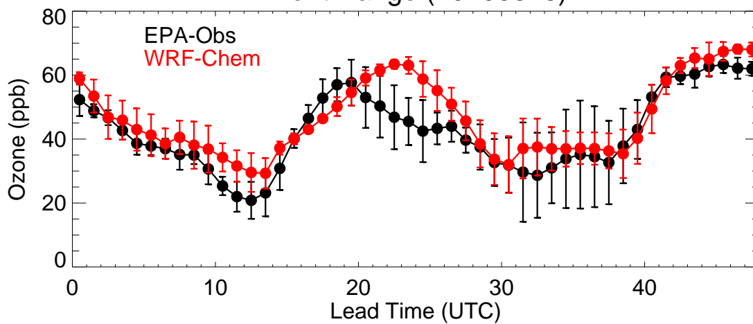
Front Range (20200626)
