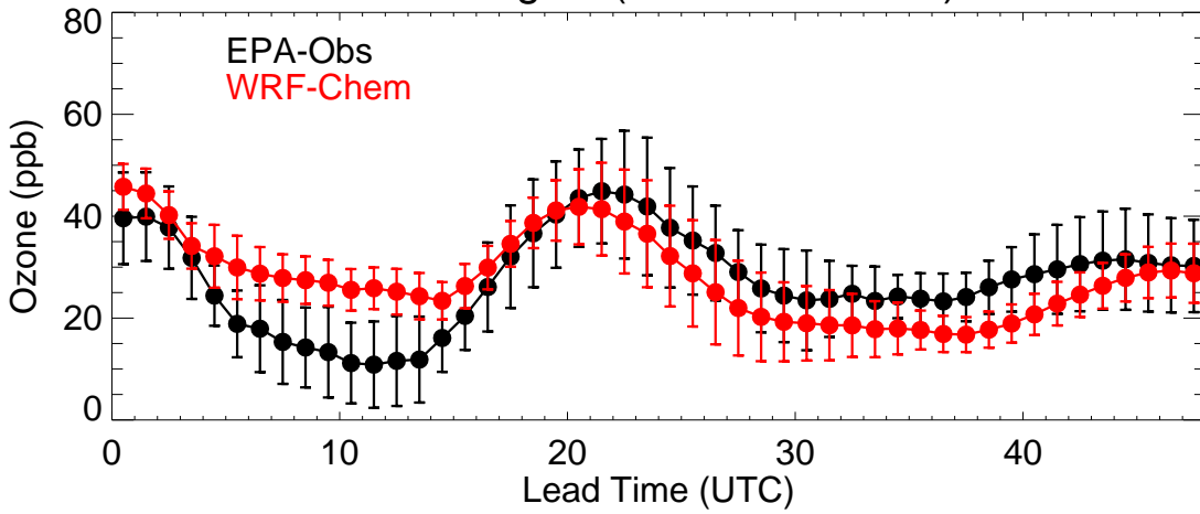
Colorado (20200626)
