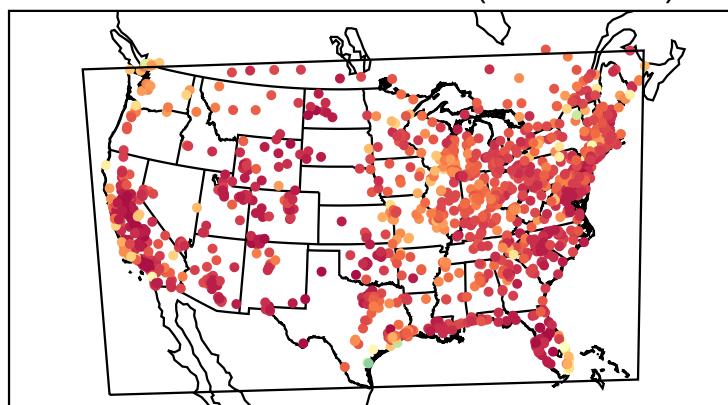
Correlation Coefficient (20200626)
