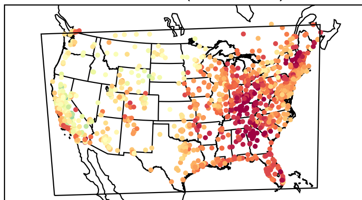
Mean Bias (20200709)
