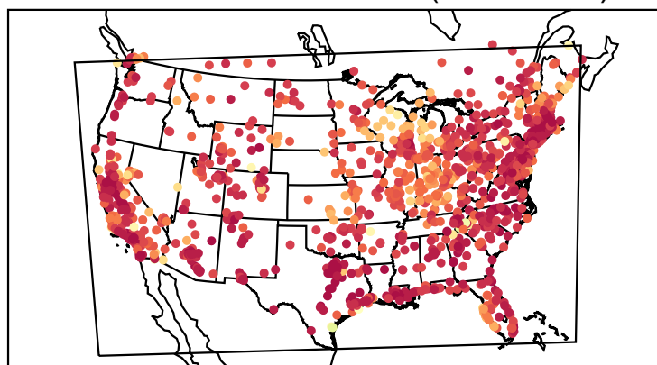
Correlation Coefficient (20200709)
