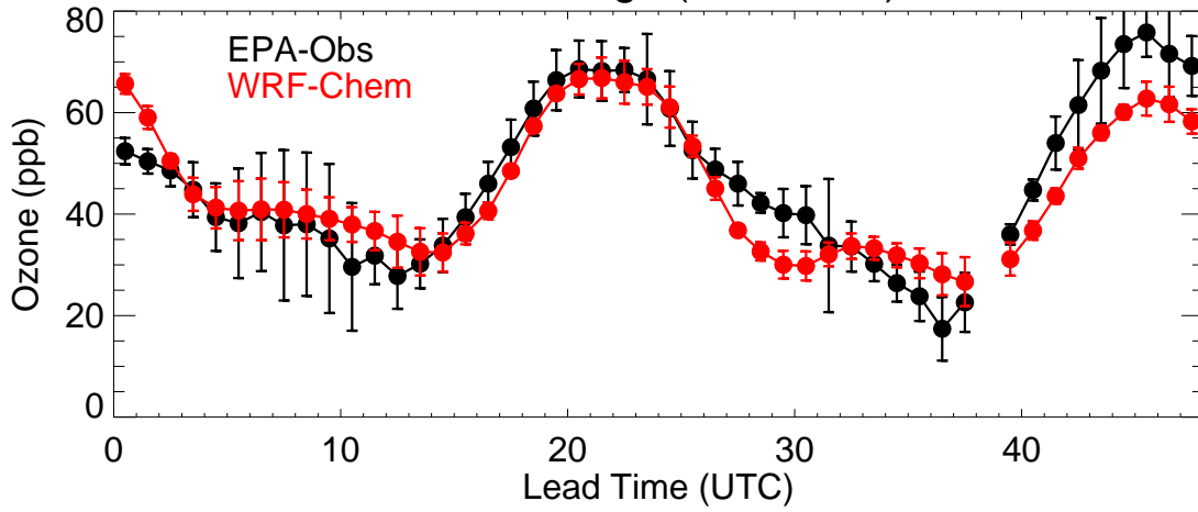
Front Range (20200802)
