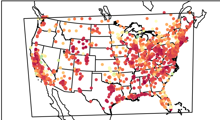
Correlation Coefficient (20200802)
