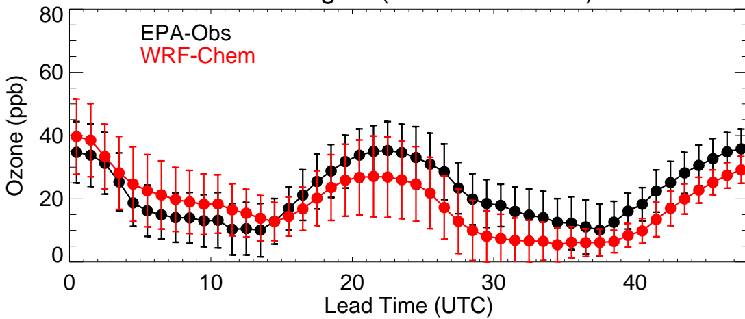
Colorado (20200802)
