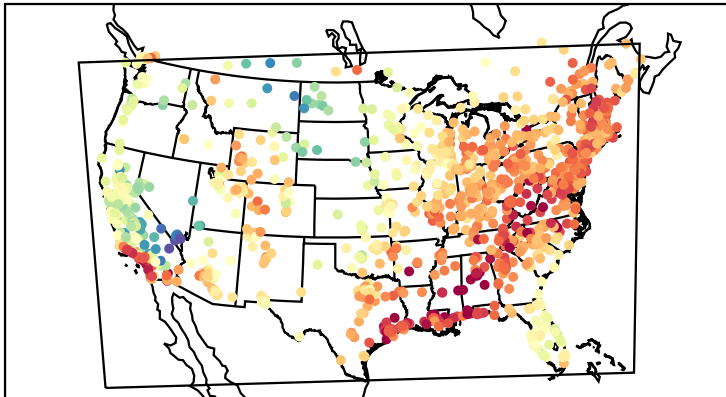
Mean Bias (20200802)
