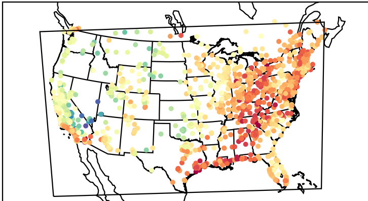
Mean Bias (20200803)
