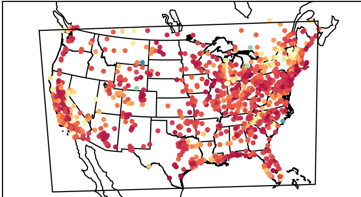
Correlation Coefficient (20200803)
