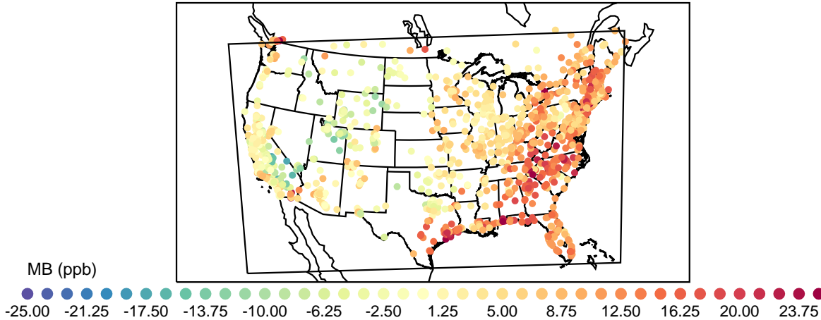
Mean Bias (20200804)
