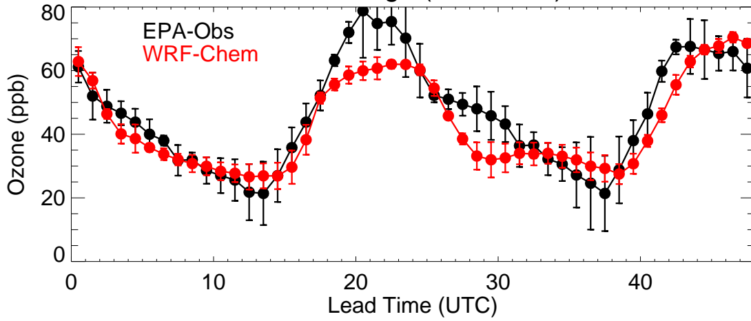
Front Range (20200804)
