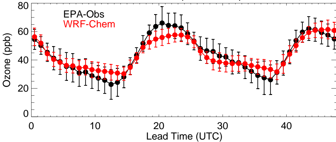
Colorado (20200804)
