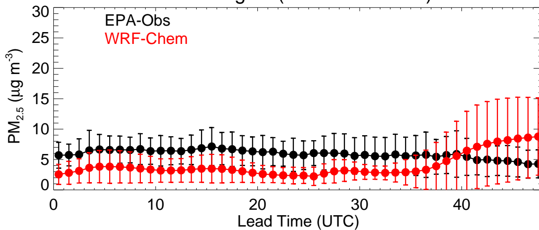
Colorado (20200805)
