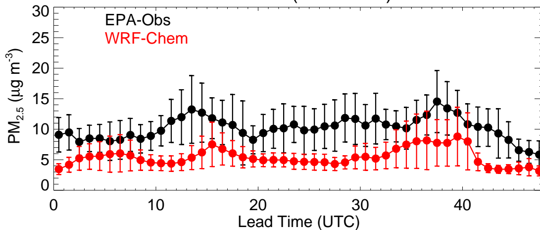
Colorado (20200805)
