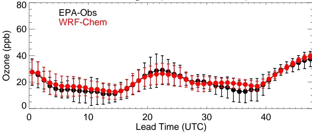
Colorado (20200821)
