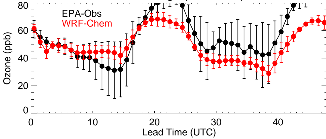
Front Range (20200821)
