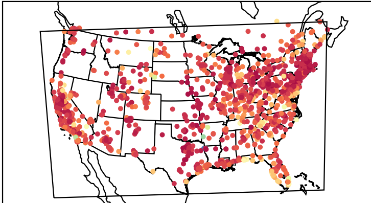
Correlation Coefficient (20200821)
