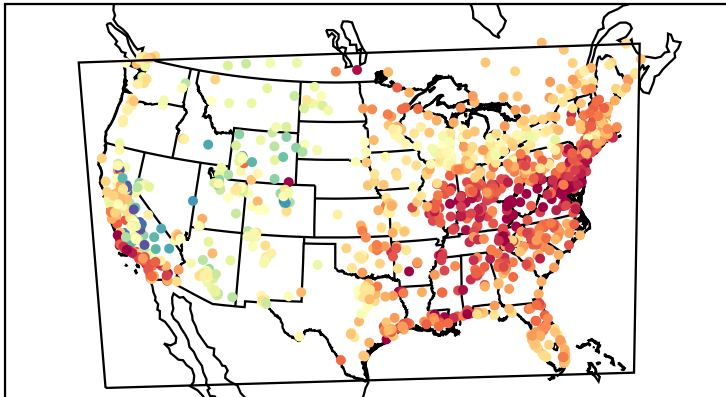
Mean Bias (20200821)
