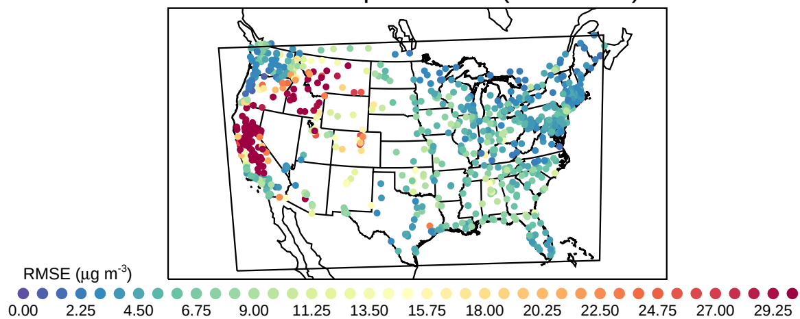
Root Mean Square Error (20200824)
