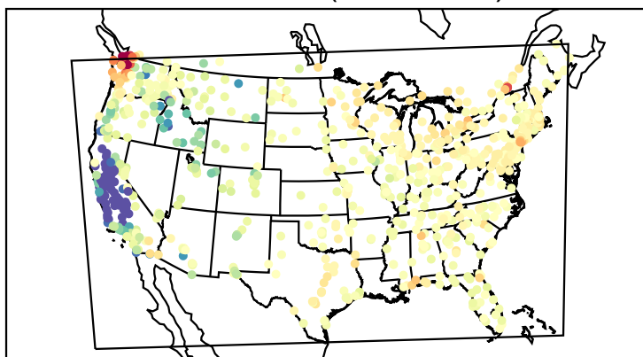
Mean Bias (20201002)
