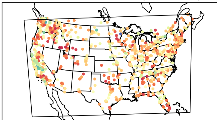
Correlation Coefficient (20201002)
