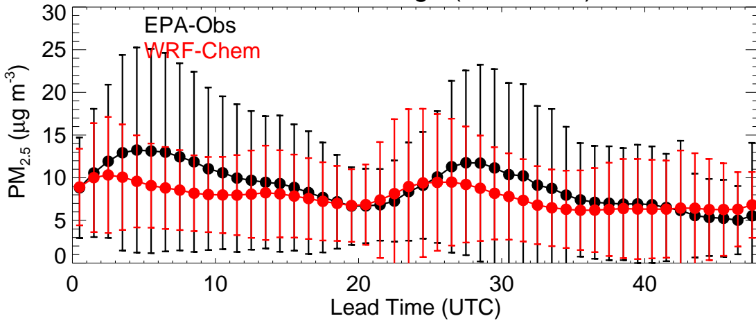
EPA Region (R1 - 20201129)
