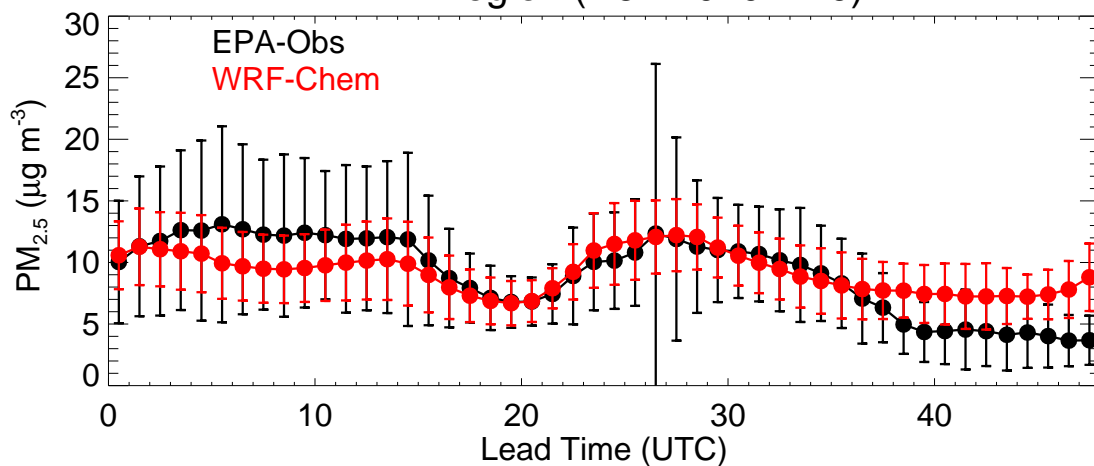
EPA Region (R4 - 20201129)
