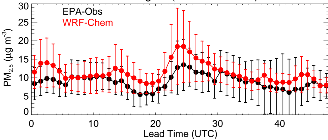
EPA Region (R2 - 20201129)
