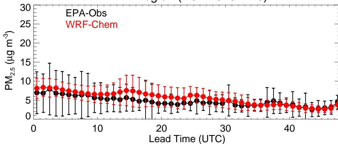
EPA Region (R7 - 20201129)
