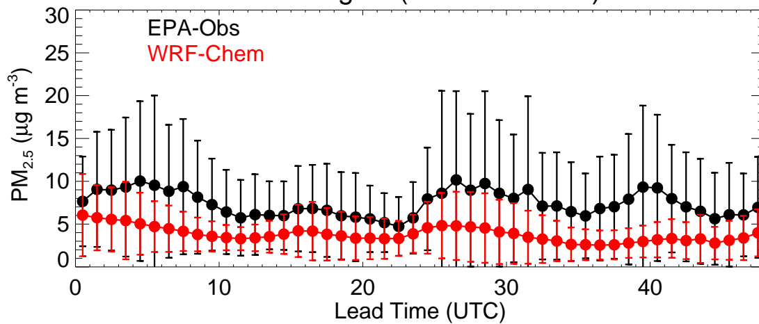
EPA Region (R8 - 20201129)
