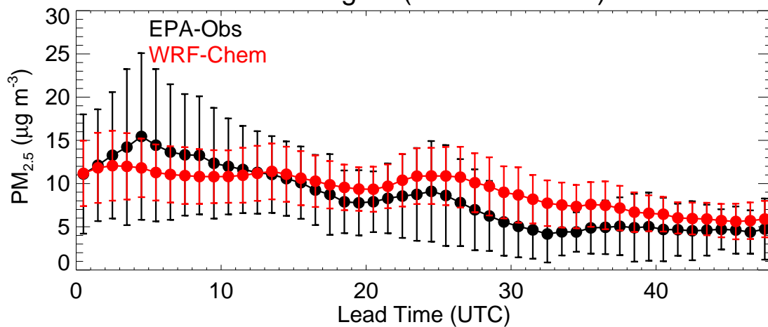
EPA Region (R5 - 20201129)
