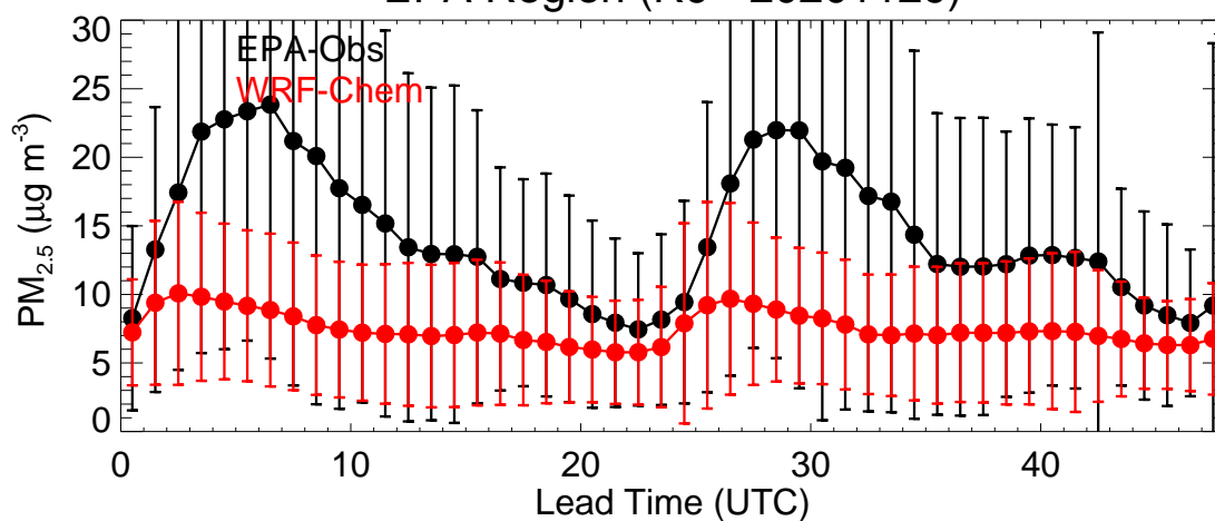
EPA Region (R10 - 20201129)
