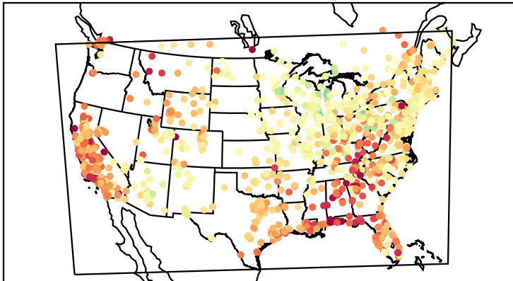
Mean Bias (20210406)
