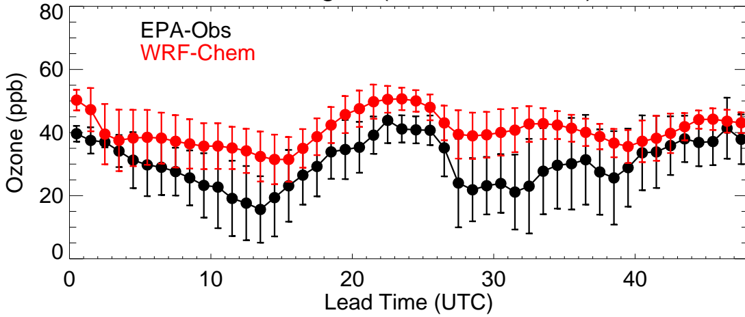
Colorado (20210406)
