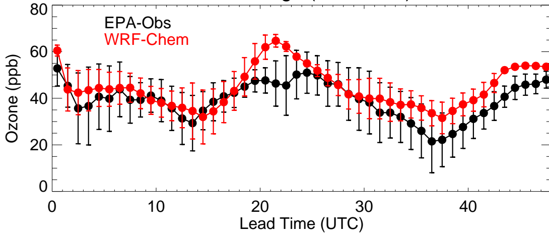
Front Range (20210406)
