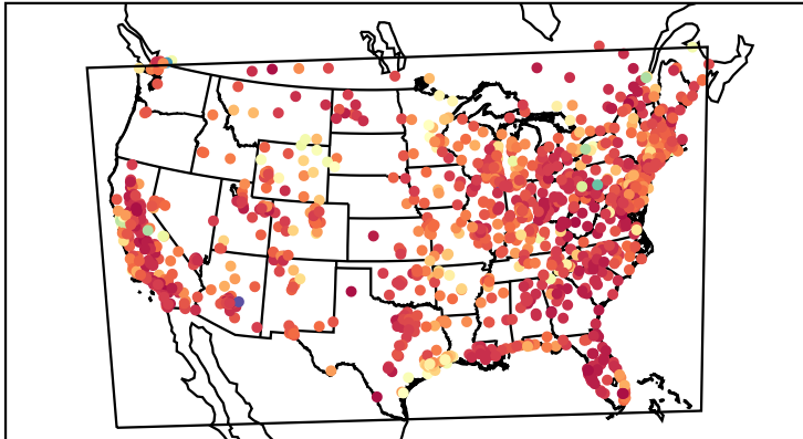
Correlation Coefficient (20210406)
