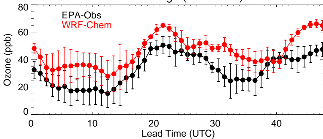
Front Range (20210517)
