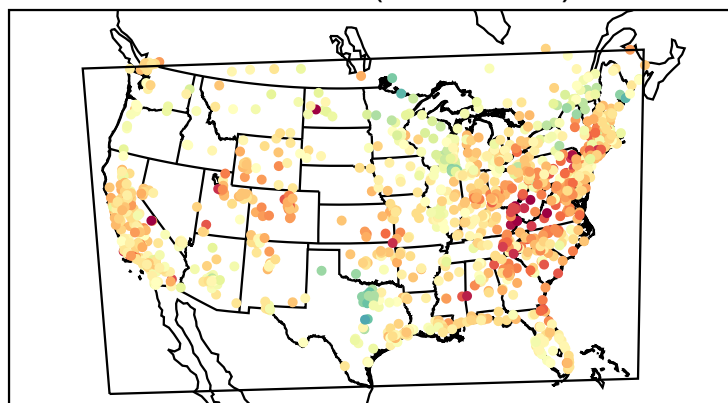
Mean Bias (20210517)
