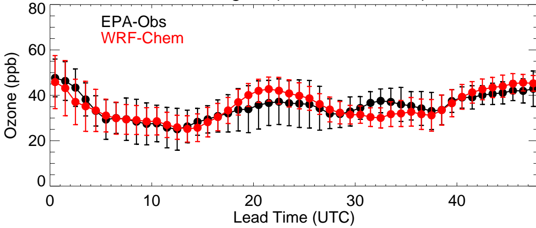
Colorado (20210517)
