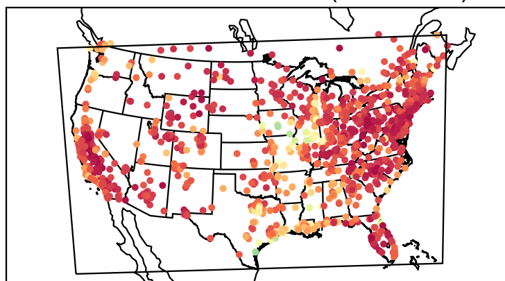
Correlation Coefficient (20210517)
