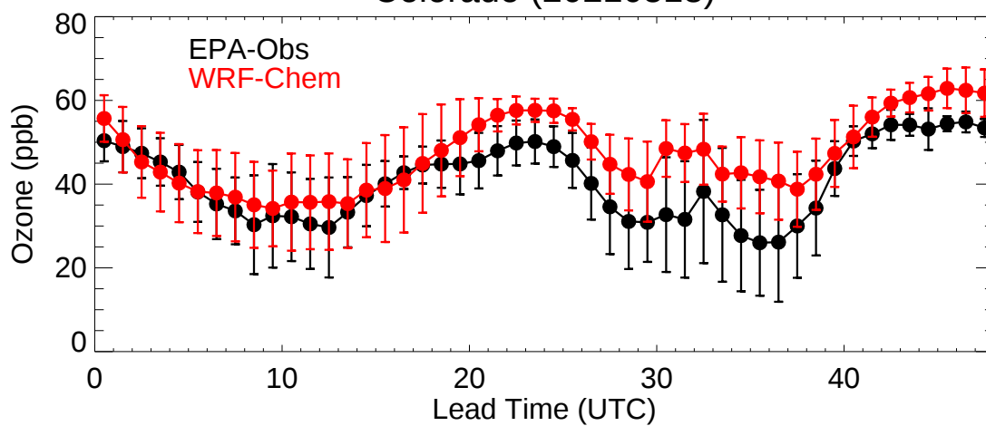
Colorado (20210518)
