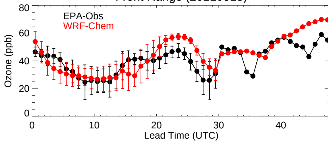
Front Range (20210518)
