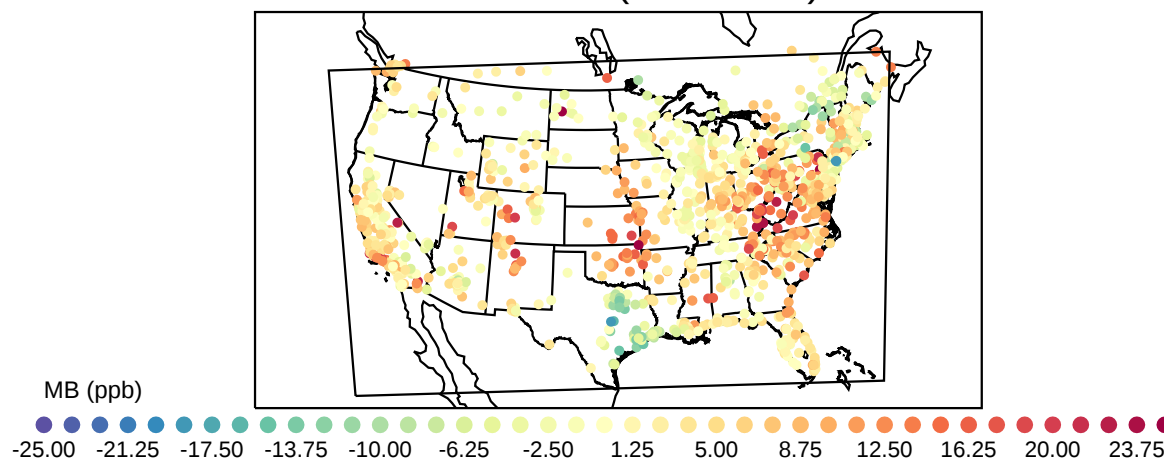
Mean Bias (20210518)
