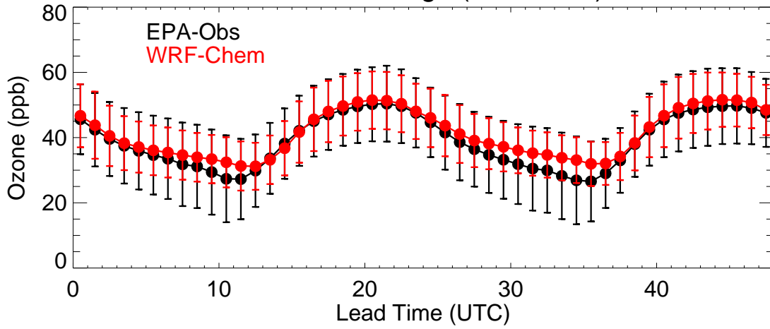
EPA Region (R1 - 20210519)
