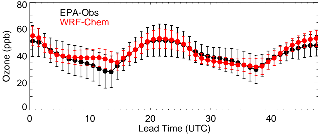
EPA Region (R10 - 20210519)
