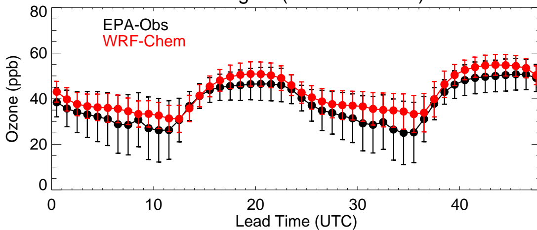
EPA Region (R5 - 20210519)
