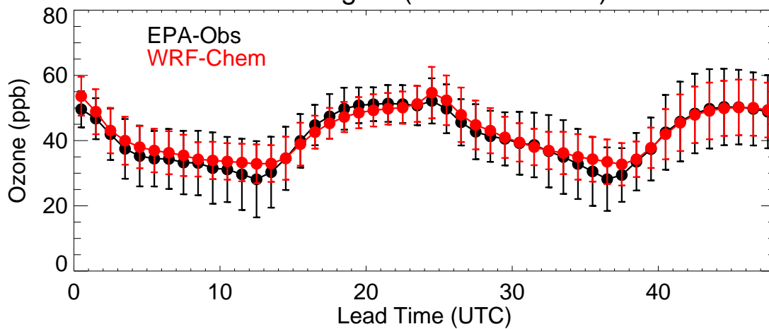
EPA Region (R8 - 20210519)
