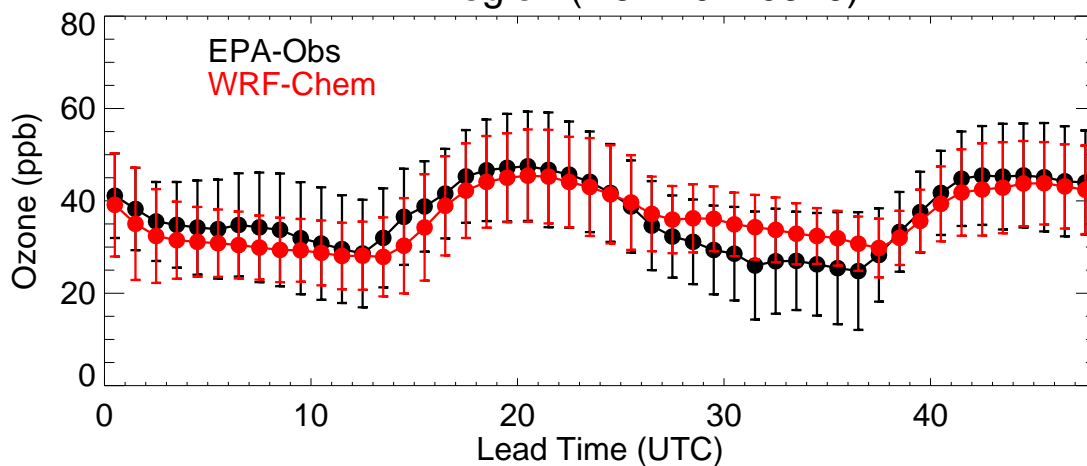
EPA Region (R7 - 20210519)
