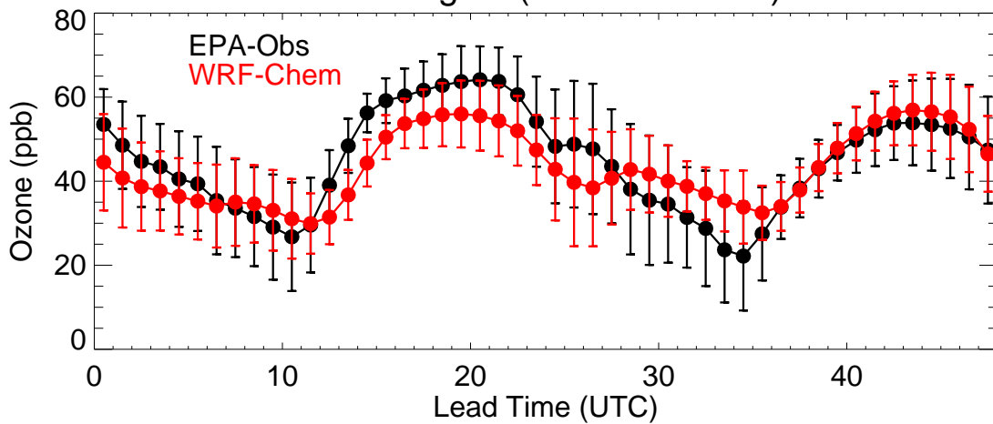
EPA Region (R2 - 20210519)
