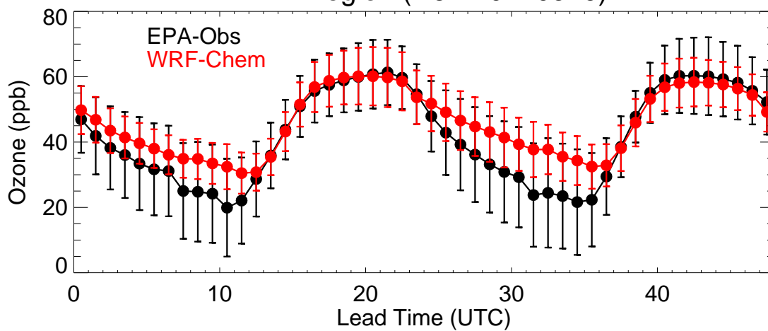
EPA Region (R4 - 20210519)
