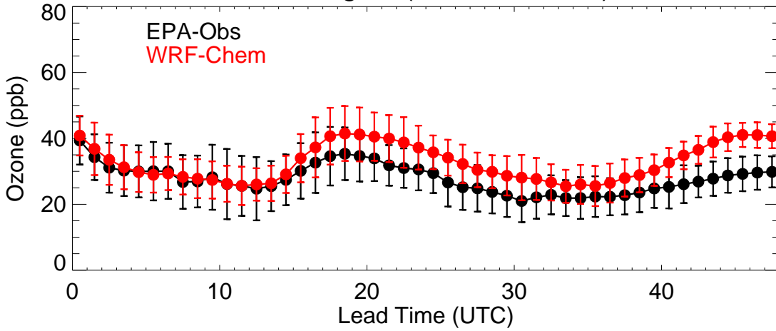
EPA Region (R8 - 20210527)
