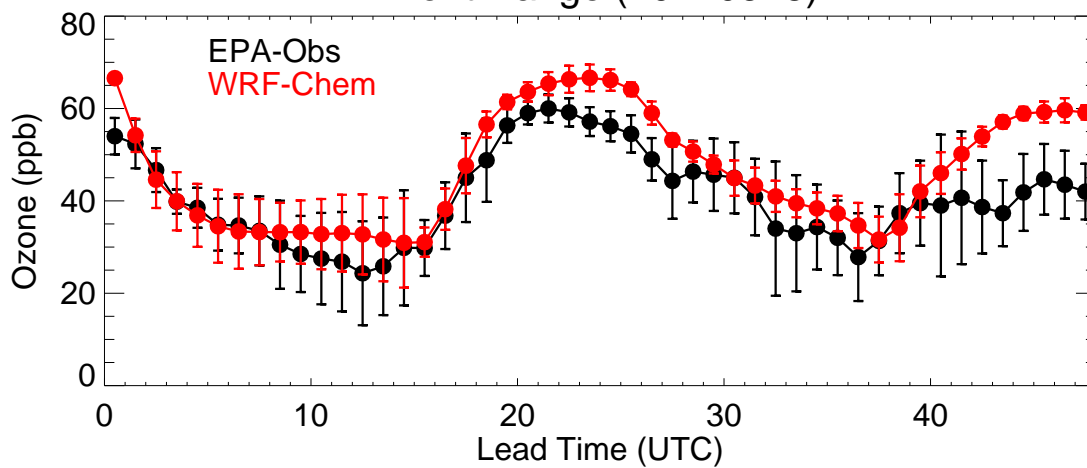
Front Range (20210528)
