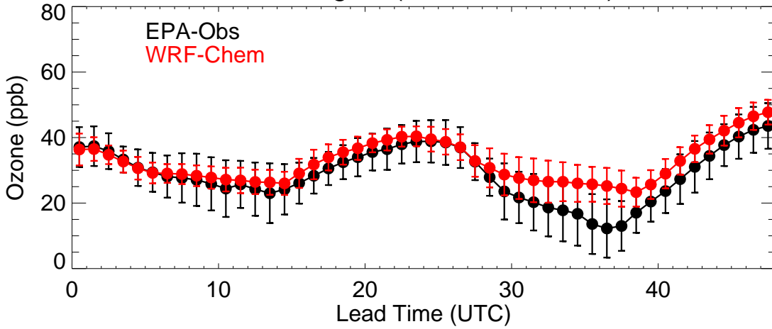
Colorado (20210528)
