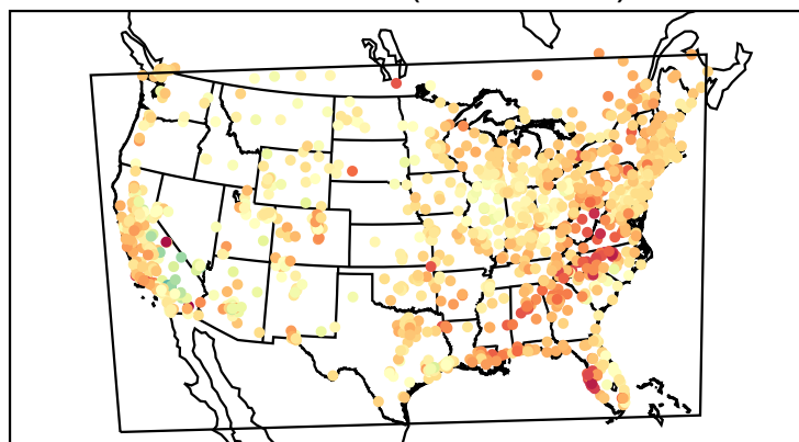
Mean Bias (20210528)
