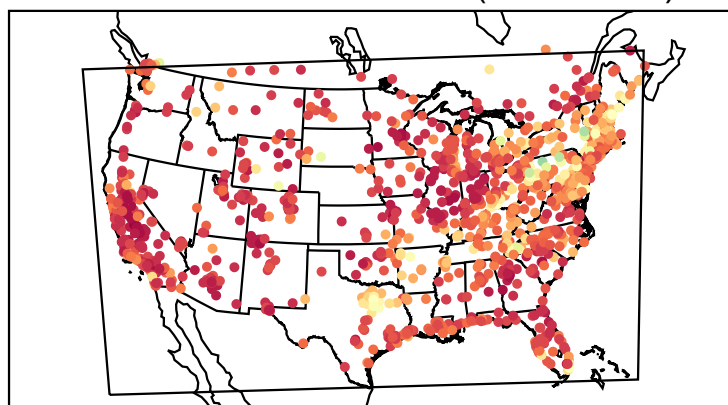
Correlation Coefficient (20210528)
