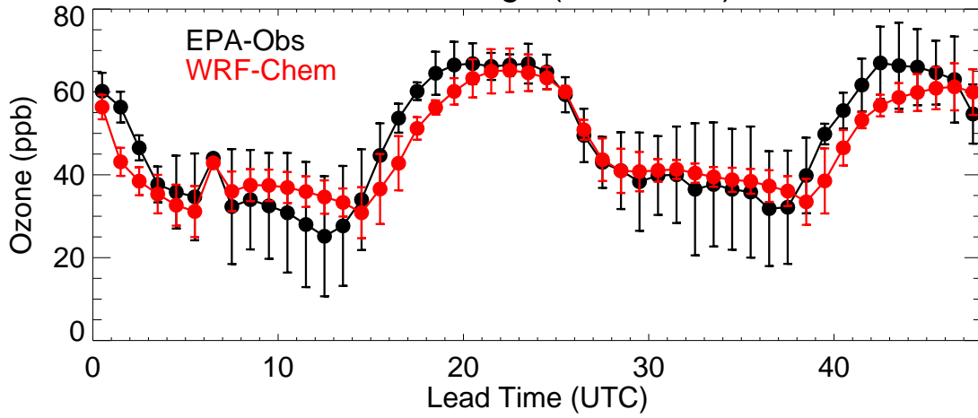
Front Range (20210604)
