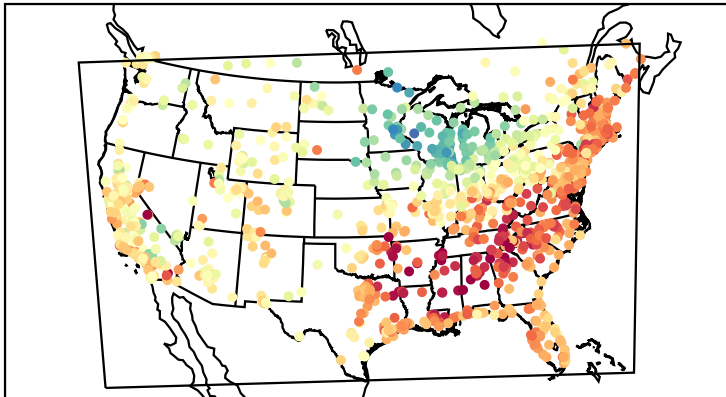
Mean Bias (20210604)
