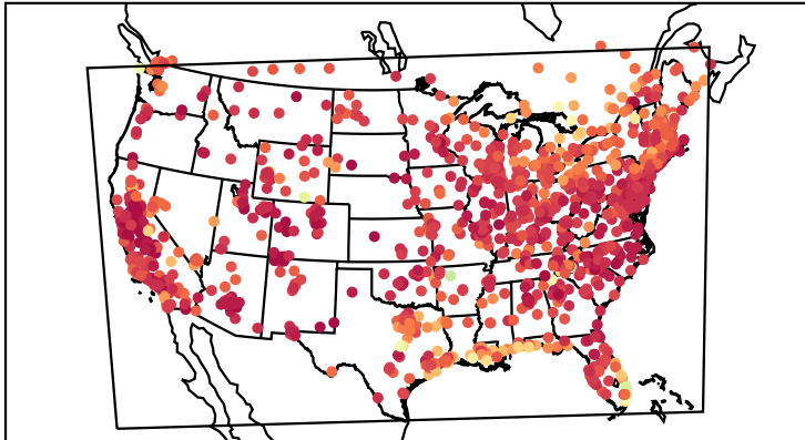
Correlation Coefficient (20210604)
