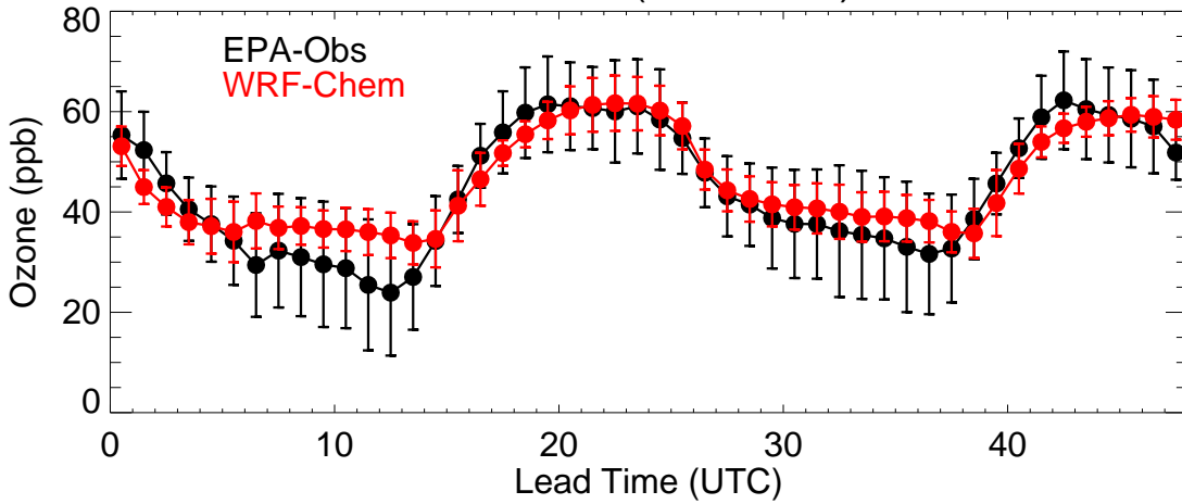
Colorado (20210604)
