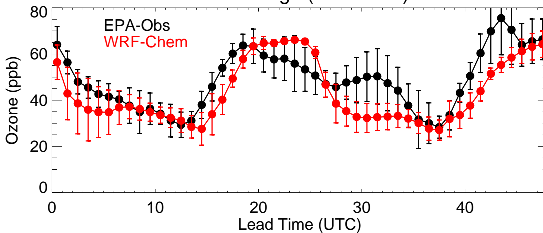
Front Range (20210613)
