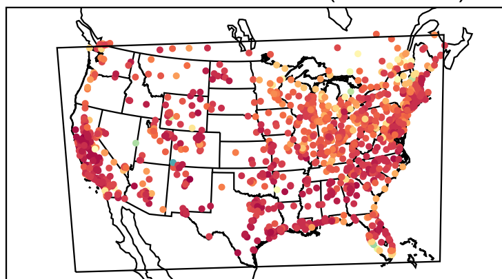
Correlation Coefficient (20210613)
