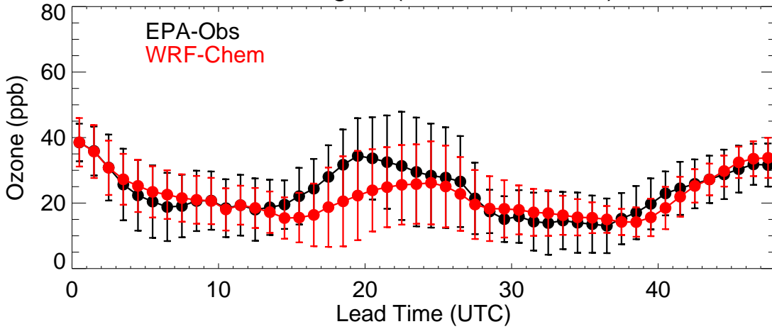
Colorado (20210613)
