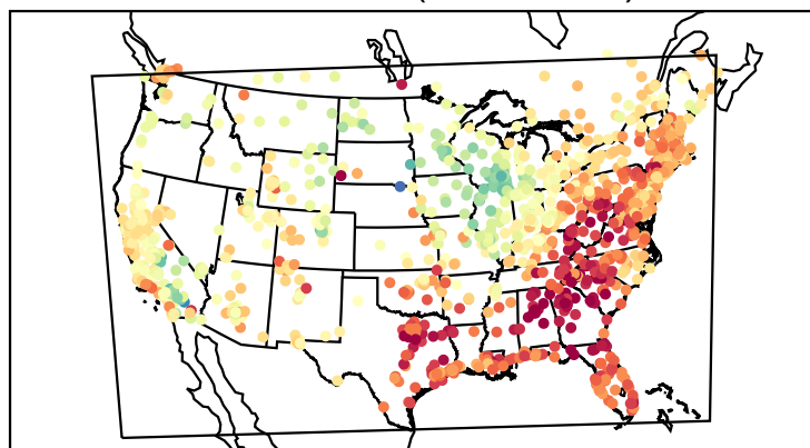
Mean Bias (20210613)
