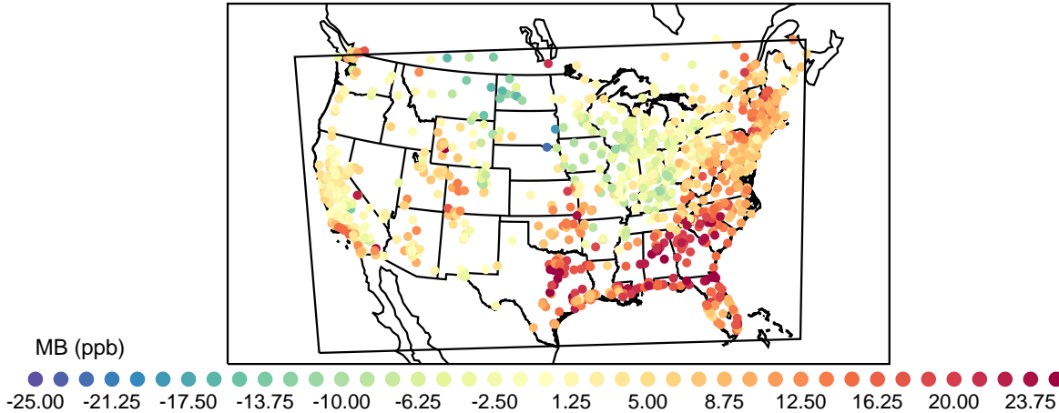
Mean Bias (20210614)
