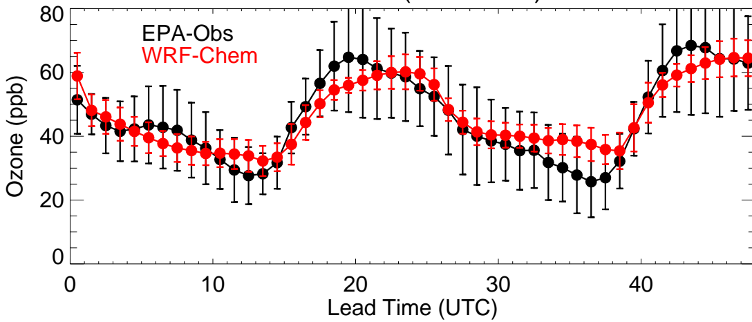
Colorado (20210614)
