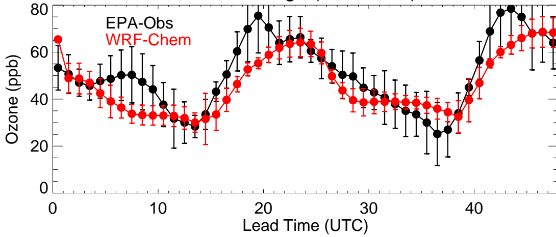
Front Range (20210614)
