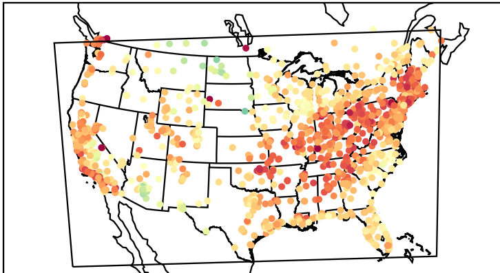
Mean Bias (20210630)
