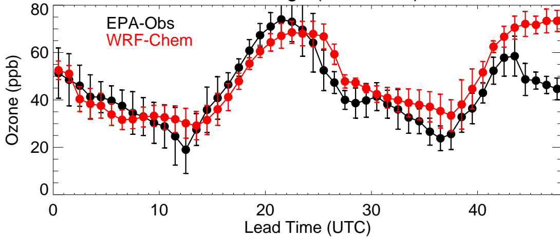
Front Range (20210630)
