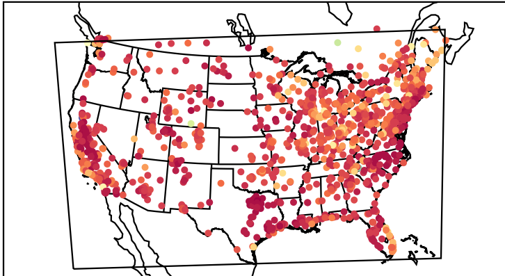
Correlation Coefficient (20210630)
