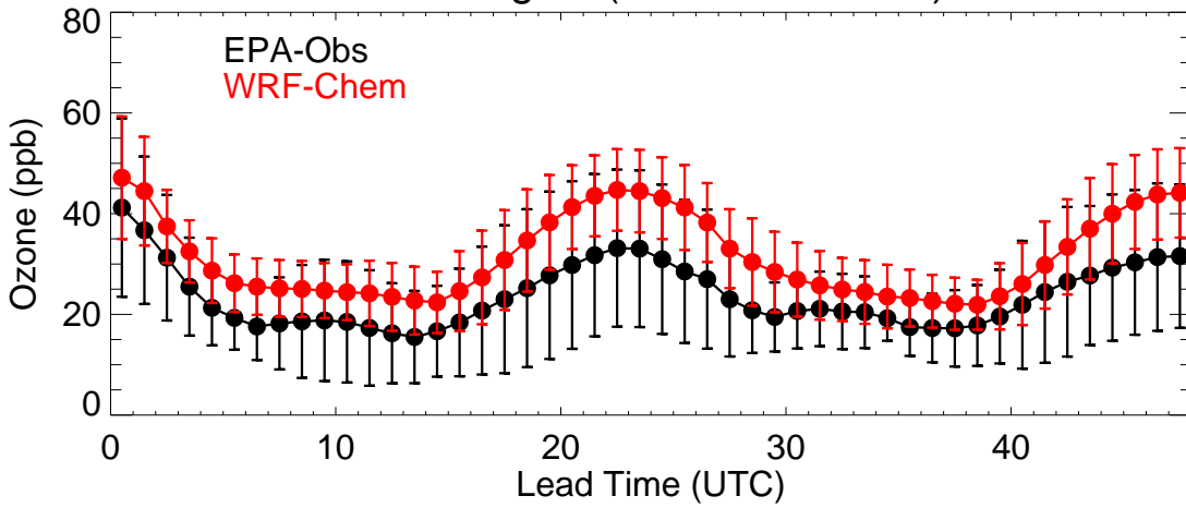
Colorado (20210630)
