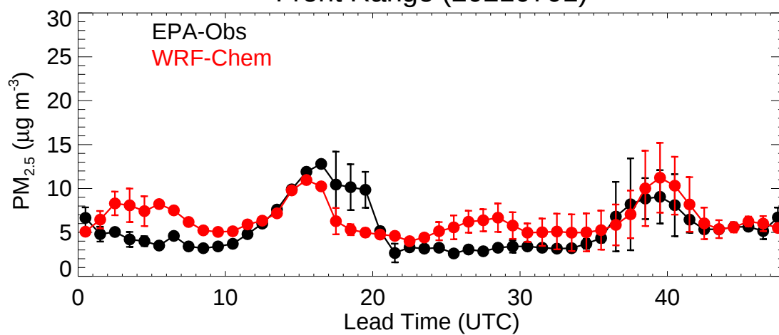
Front Range (20210701)
