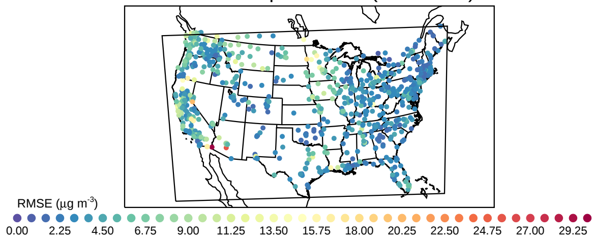
Root Mean Square Error (20210701)
