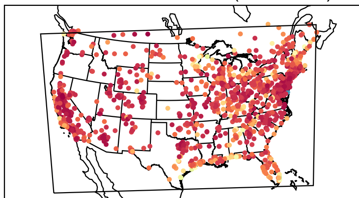
Correlation Coefficient (20210706)
