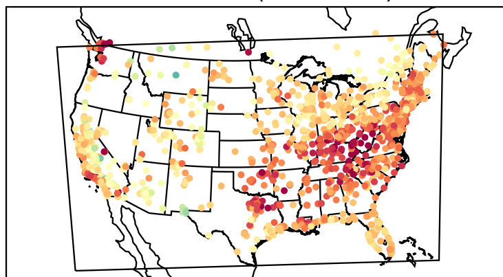
Mean Bias (20210706)
