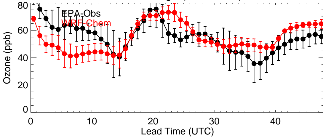
Front Range (20210713)
