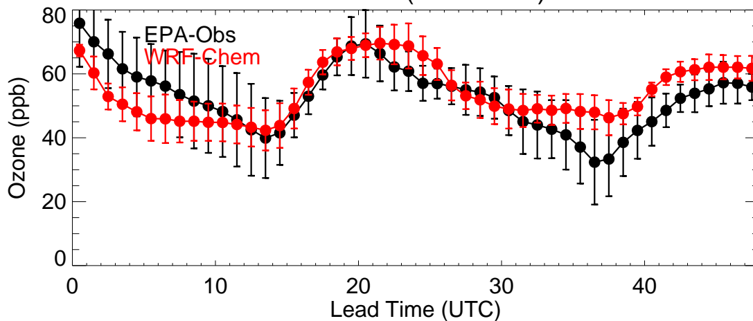
Colorado (20210713)
