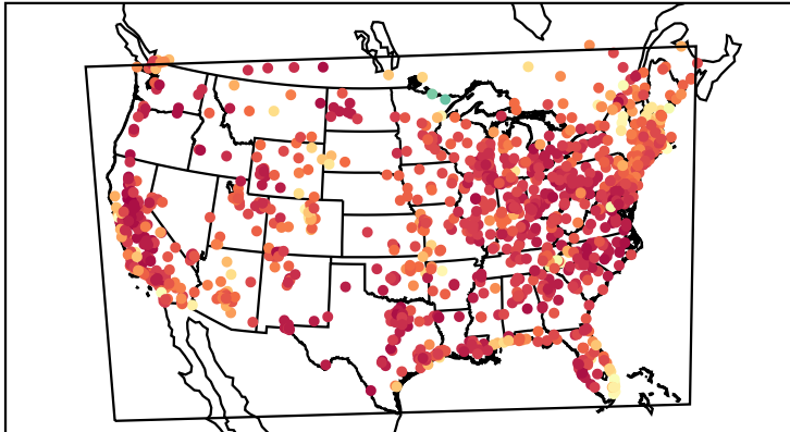
Correlation Coefficient (20210713)
