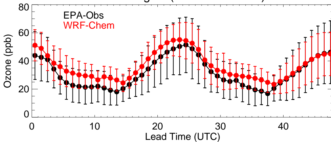
Colorado (20210713)
