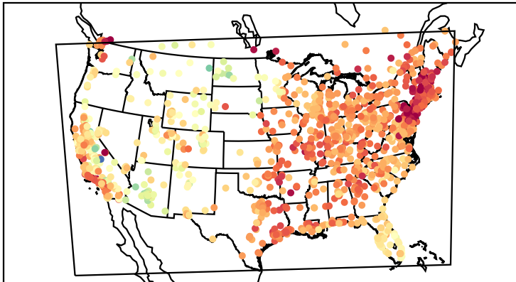
Mean Bias (20210713)
