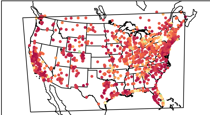
Correlation Coefficient (20210716)
