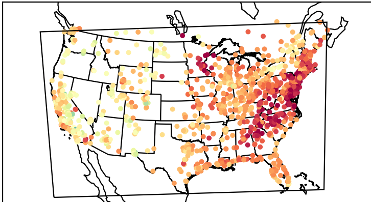
Mean Bias (20210716)
