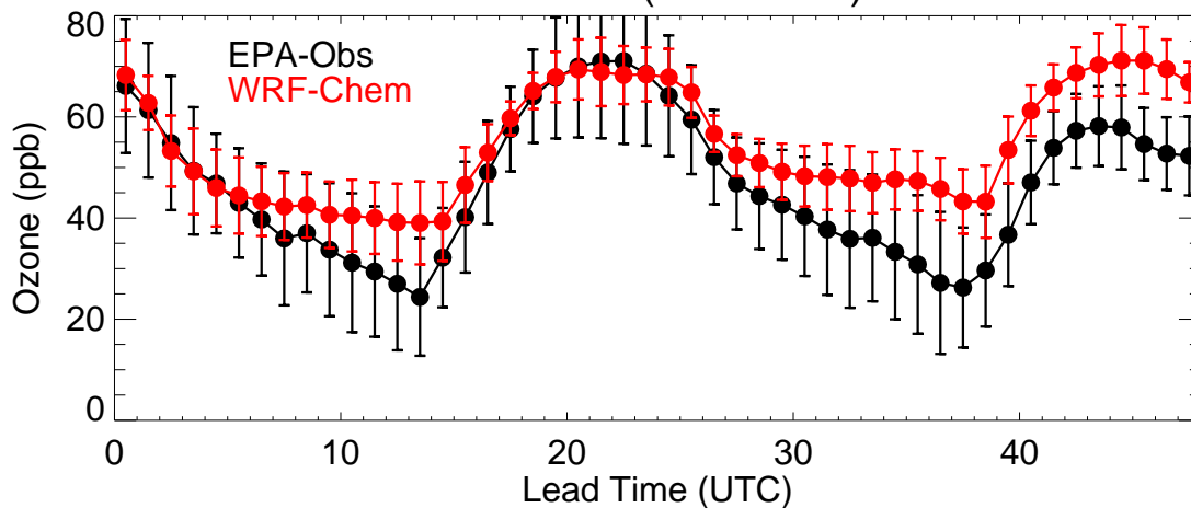
Colorado (20210802)
