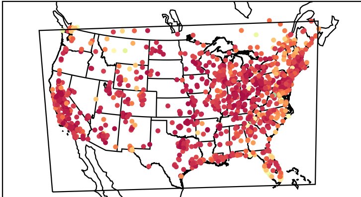
Correlation Coefficient (20210802)
