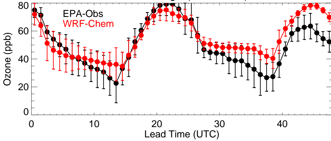
Front Range (20210802)
