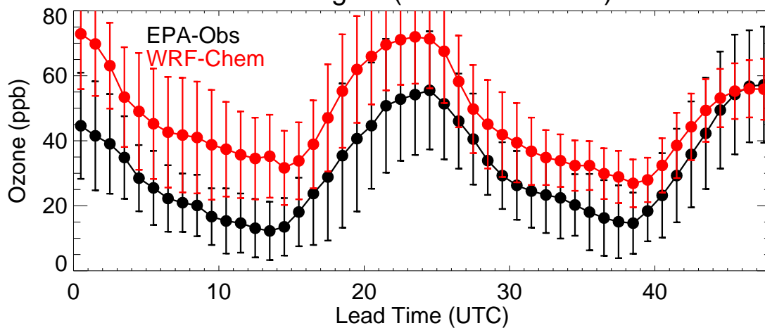
Colorado (20210802)
