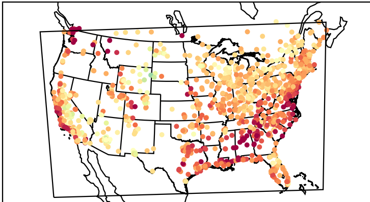
Mean Bias (20210802)
