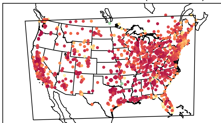
Correlation Coefficient (20210804)
