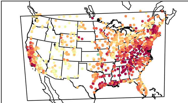
Mean Bias (20210806)
