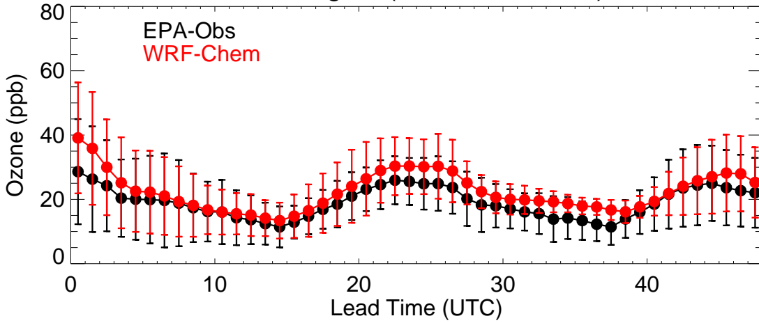
Colorado (20210806)
