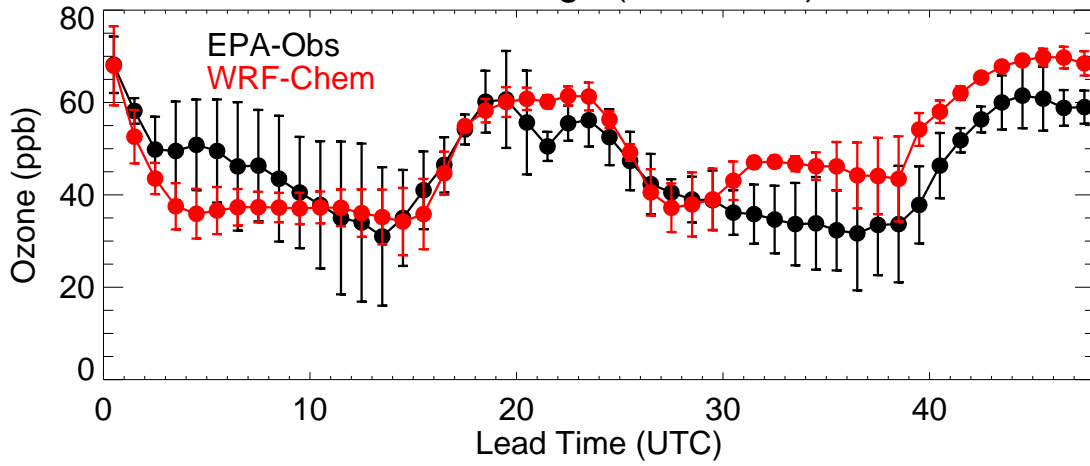
Front Range (20210806)
