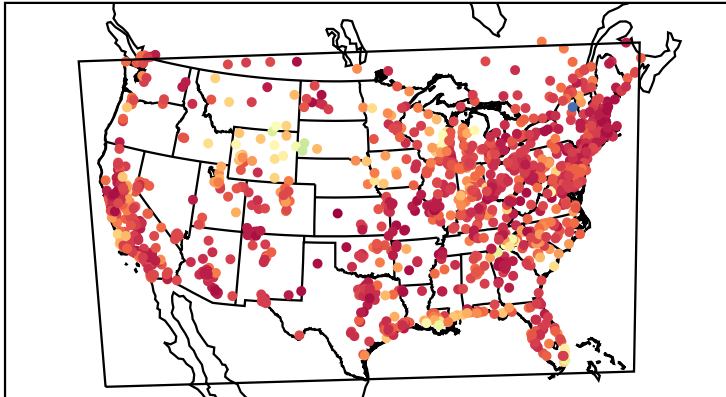
Correlation Coefficient (20210806)
