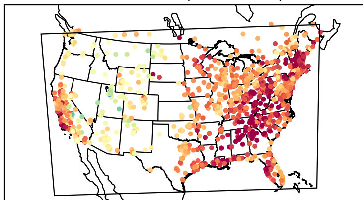
Mean Bias (20210807)
