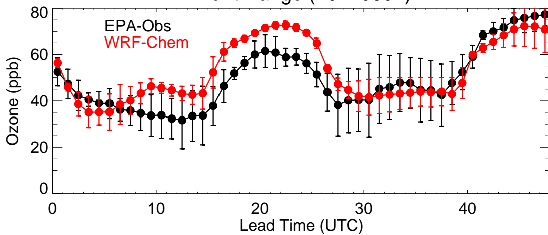
Front Range (20210807)
