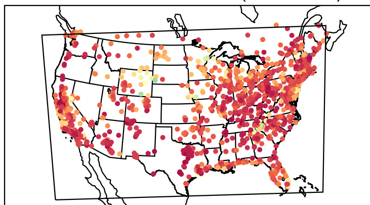
Correlation Coefficient (20210807)
