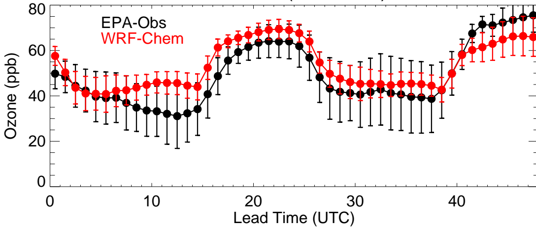
Colorado (20210807)
