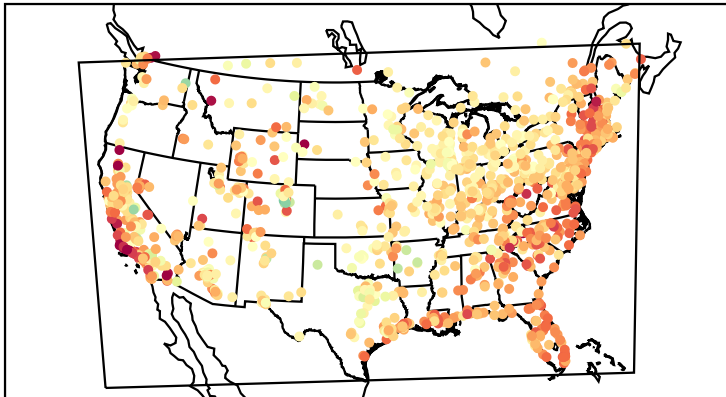
Mean Bias (20210909)
