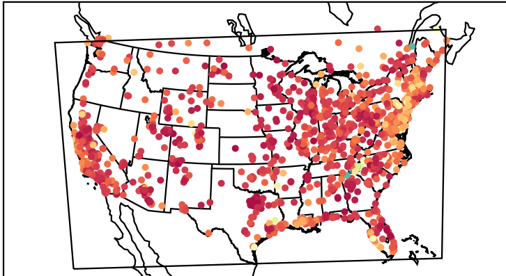
Correlation Coefficient (20210909)
